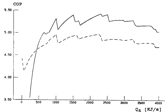
Figure 4. COP for an optimized design of the plant (with advanced management) with increasing load in the -6^{\circ}\text{C} system. August. (—) : Q_{10} = 0 \text{ KJ/s} . (---) : Q_{10} = 1000 \text{ KJ/s} .
