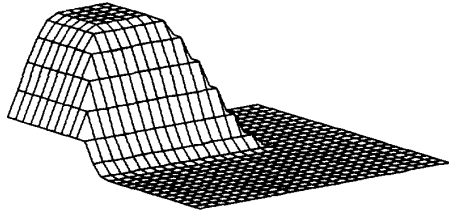
Fig. 5 The 2-dimensional fuzzy set "upper slightly left".
