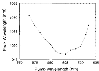
QMG3 Fig. 2. The peak wavelength of the superfluorescence emission versus pump wavelength for the double-pass configuration.
