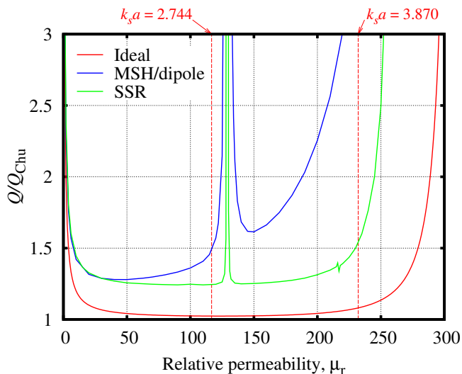
Fig. 6. Ratio Q/Q_{Chu} for the spherical split ring (SSR) antenna with magnetic core.
