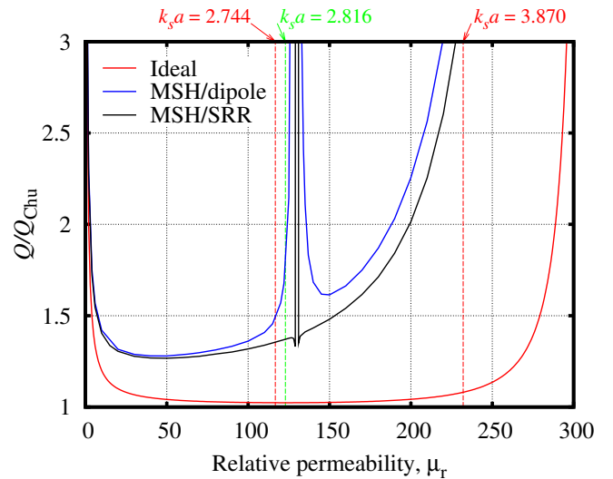
Fig. 3. Ratio Q/Q_{\text{Chu}} for an ideal \text{TE}_{10} -mode antenna and numerical results for the MSH antenna with dipole and SRR excitation.
