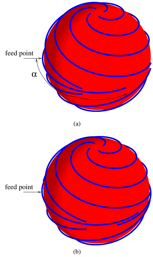
Fig. 2. Multiarm spherical helix (MSH) antenna with magnetic core excited by (a) a curved dipole [3] and (b) a split-ring resonator (SRR).
