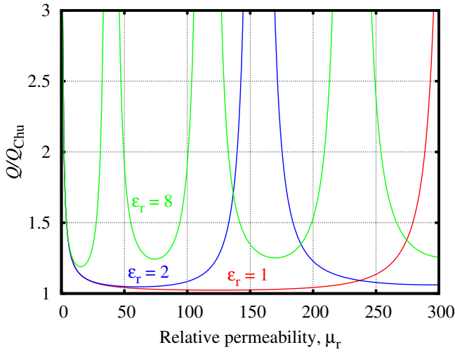
Fig. 1. Theoretical ratio Q/Q_{\text{Chu}} versus the core permeability \mu_r for ka = 0.254 and three values of the core permittivity \epsilon_r = 1, 2, 8 .
