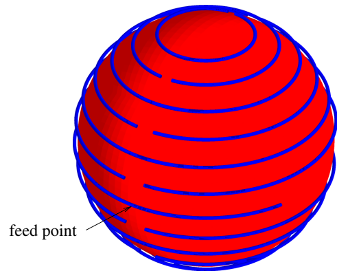
Fig. 5. Spherical split ring (SSR) antenna with magnetic core.
