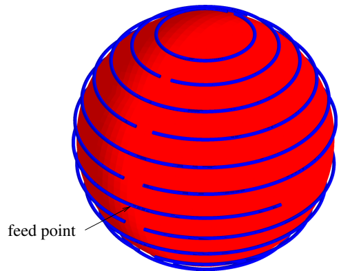
Fig. 5. Spherical split ring (SSR) antenna with magnetic core.
