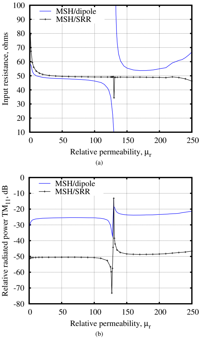
Fig. 4. Input resistance at resonance (a) and the relative radiated power of the TM_{11} mode (b) of the MSH antenna with magnetic core excited by a curved dipole and an SRR.
