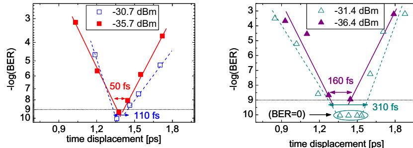
Figure 5. Timing tolerance at 640 Gbit/s, measured at the receiver sensitivity and at 5 dB more power to the receiver. Left: 700 fs gaussian control pulse. Right: 840 fs FT control pulse giving up to 310 fs tolerance with BER = 0.
