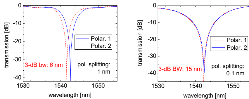
Figure 2. Bandwidth and polarisation. Left: LPG used in [6] with 6 nm width and a 1 nm polarisation splitting. Right: New LPG for this work with 15 nm bandwidth and only 100 pm polarisation splitting.
