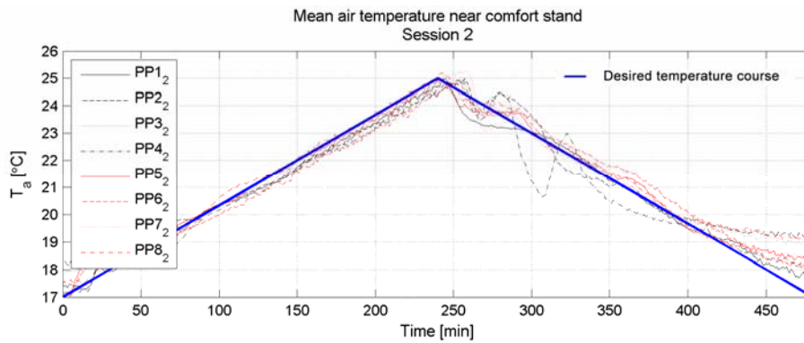
Figure 2. Desired and measured temperature course during experiment.
