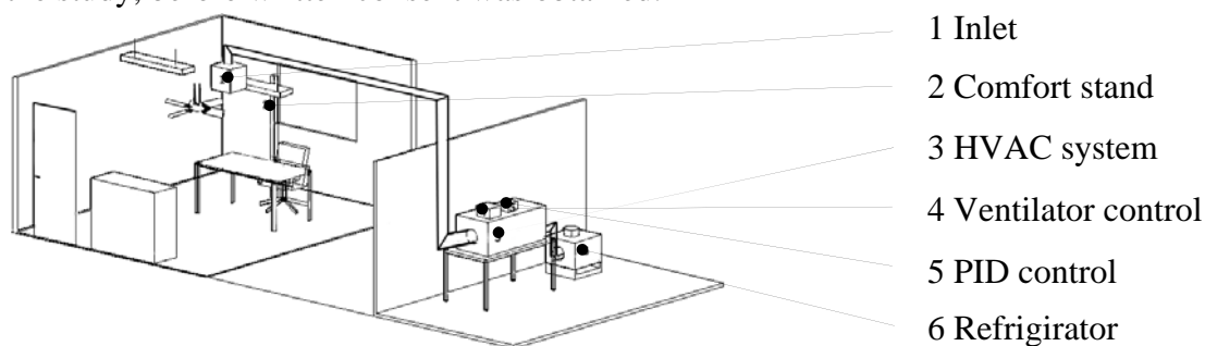
Figure 1. Schematic drawing of the climate room.
