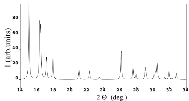
FIG. 3. The XRD diffraction pattern for LiBH_4 with Cc symmetry. The diffraction pattern is given for a beam wave length of \lambda = 0.949 Å.
