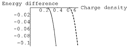
FIG. 2. The normalized energy difference \Delta_n from Eq. (49) for the ellipselike n=2 (solid line) and triagonlike chain n=3 (dashed line) with 2\chi=4 J=k .
