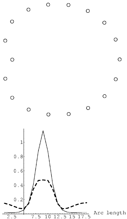
FIG. 6. Same as Fig. 5 with \nu=0.23 , \chi=2.15 , k=J=1 .
