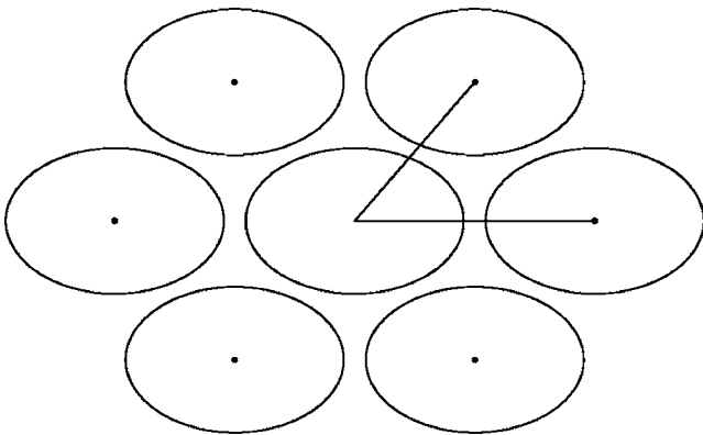
FIG. 8. Arrangement of densely packed ellipselike aggregates.
