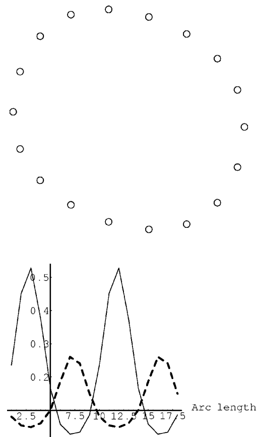
FIG. 4. The top panel shows the equilibrium shape of the chain and the bottom panel shows the charge distribution (solid line) and curvature variation (dashed line) along the chain in the case of hardening electron-curvature interaction with \nu=0.22 , \chi=-2 , k=1 , J=0.4 .
