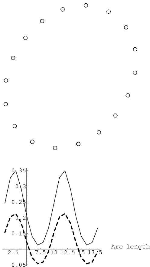
FIG. 5. The top panel shows the equilibrium shape of the chain and the bottom panel shows the charge distribution (solid line) and curvature variation (dashed line) along the chain in the case of softening electron-curvature interaction with \nu=0.22 , \chi=2.15 , and k=J=1 .
