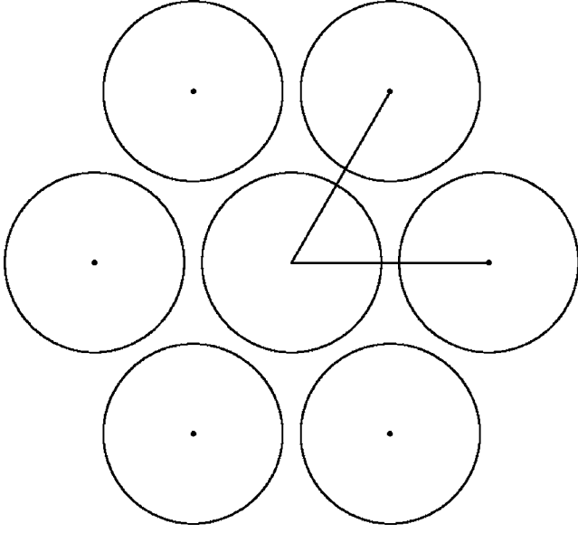
FIG. 7. Arrangement of densely packed ringlike aggregates.
