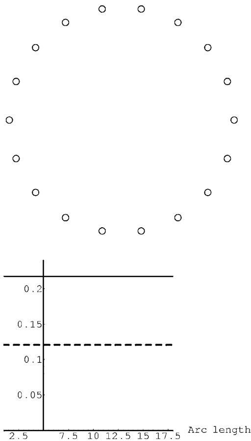
FIG. 3. The top panel shows the initial shape of the chain; the bottom panel shows the initial charge (solid line) and curvature (dashed line) distribution along the chain.
