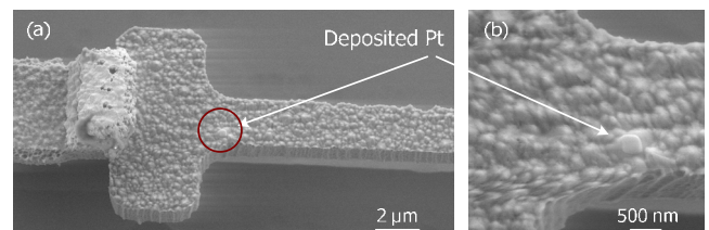
FIG. 4. (Color online) SEM images of mass loaded resonator where the Pt compound has been deposited. The volume of the Pt deposit is estimated as a square of side length 370 nm with a thickness of 340 nm. This yields an estimated mass loading of 484 \pm 91 fg.
