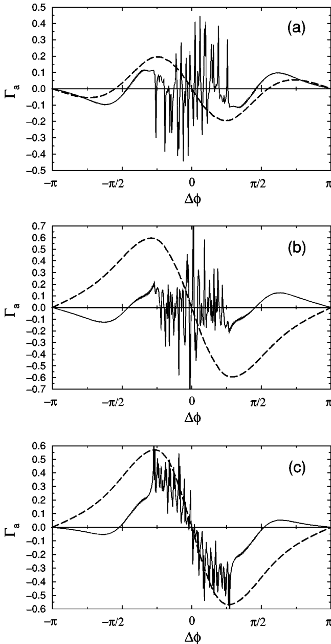
FIG. 10. Effective coupling function for the multispike bursting regimes. The solid line is for V coupling while the dashed line is for S coupling (a) seven spikes per train at k_S = 0.00011 ; (b) eight spikes per train at k_S = 0.00009 ; (c) nine spikes per train at k_S = 0.00008 . Note, how the slow variation of \Gamma_a in (c) causes the number of stable synchronization regimes to be quite small, even for V coupling.
