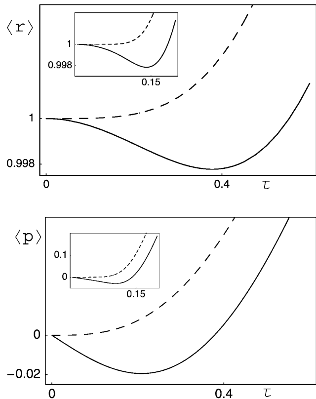
FIG. 1. Comparison between the time evolutions of a circular (solid line) and a spherical shell (dashed line) using the average radial position (top) and the average radial momentum (bottom) obtained from Eqs. (3) and (9) for a^{(2)} = 15/7 and a^{(3)} = 2 . On average the two-dimensional shell first contracts and then expands, whereas the three-dimensional one expands from the onset. In the left insets we show the short time behavior of a displaced Gaussian radial wave packet obtained numerically. Here we have used the same Gaussian for an initial radial wave function in two and three dimensions with \delta r = 0.4 and \rho = 1.5 in arbitrary units. Position is scaled in units of the initial position r_0^{(N)} of the wave packet and momentum in terms of the final momentum p_\infty^{(N)} .
