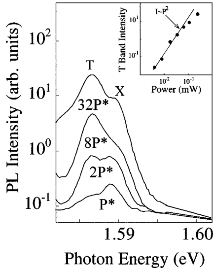
FIG. 3. Photoluminescence spectra at T=11 K for different exciting power density ( P^* = \text{W cm}^{-2} ). The peak intensity of the T band as a function of the excitation power is reported in the inset (the full line corresponds to a quadratic dependence of intensity on power).
