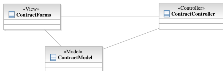
Figure 2: Components of the Model-View-Controller pattern
