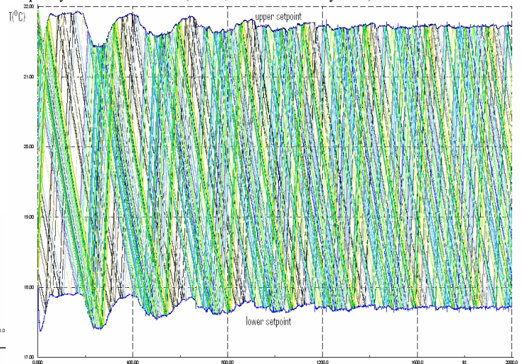
Fig 11 The aggregated heater (100 units) simulation results of heater temperatures with DFR function (kf=15, 70% units initially “on”)
