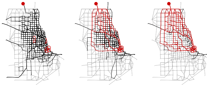
a) b) c) a) shows the ChicagoSketch with no demand alteration. On b) the demand has been intensified and on c) the network is practically flushed from the designated origin. The black sections are sections which are used by o/d-pairs that splits the flow between two paths. The red sections used by o/d-pairs that uses three or more different paths. The filled red circle is the origin where the flow is inserted and the outlined circles are the destinations.
