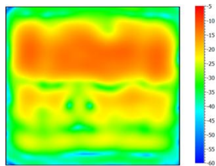
Figure 4 - Amplitude of the y-component of the tangential electric field from traditional microwave holography.
