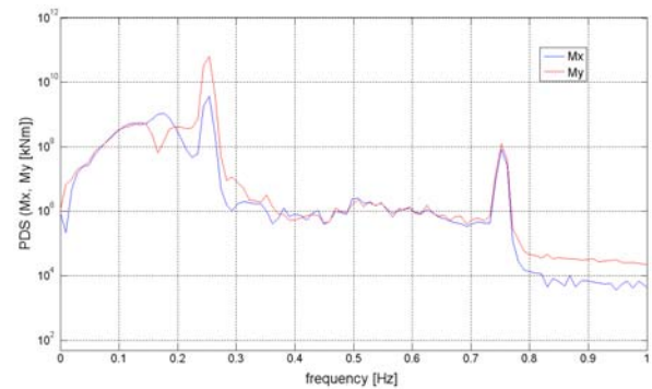
Figure 15 Density power spectrum of the bending moments M_x , M_y , at the water surface plane
