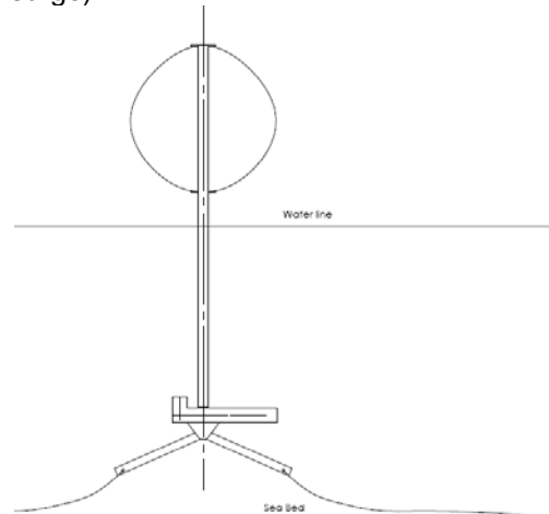
Figure 4 Schematic drawing of the third configuration (Mooring fixed configuration)
