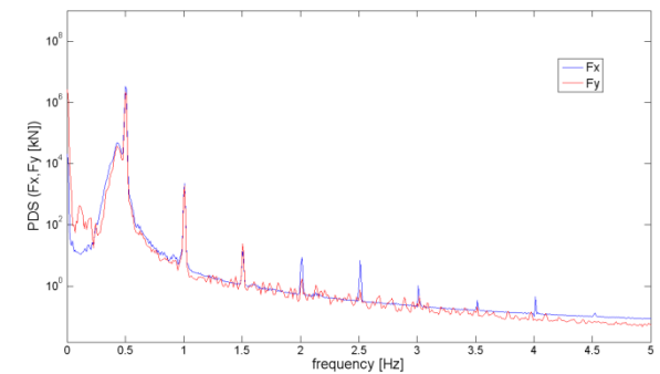
Figure 16 Density power spectrum of the force on the rotor, F_x , F_y
