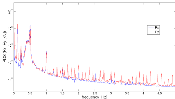
Figure 29 Density power spectrum of the force on the rotor, Fx, Fy
