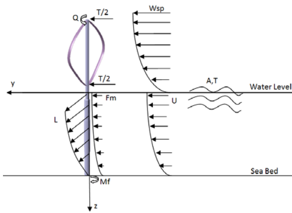
Figure 5 External conditions and main loads on the turbine
