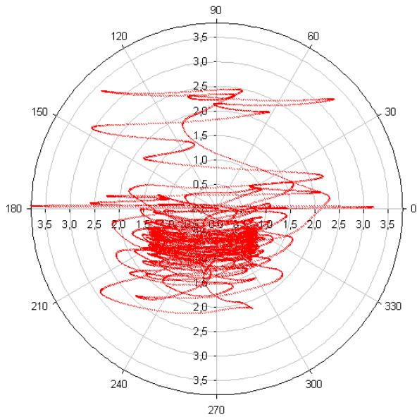
Figure 18 Trajectory of the surface section of the tower in the water surface plane xy
