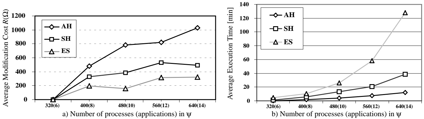
Figure 6. Average Modification Cost (a) and Execution Time (b) for MS with the AH, SH and ES Approaches to Subset Selection
