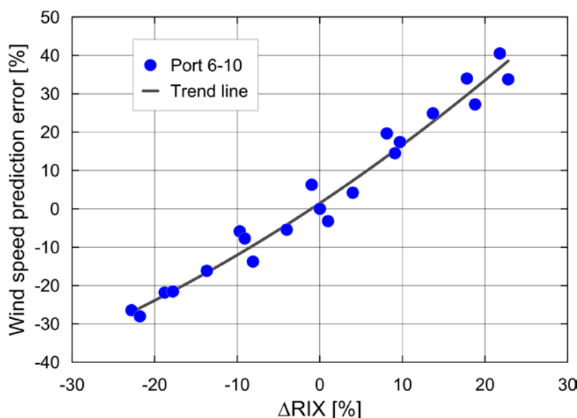
Figure 17. WAsP wind speed prediction error in per cent as a function of the difference in ruggedness indices, \Delta RIX [\%] , between the predicted site and the predictor site. Data points represent cross-predictions between 5 masts in N Portugal. RIX values were calculated using the WAsP default set-up; other values may provide a better fit.
