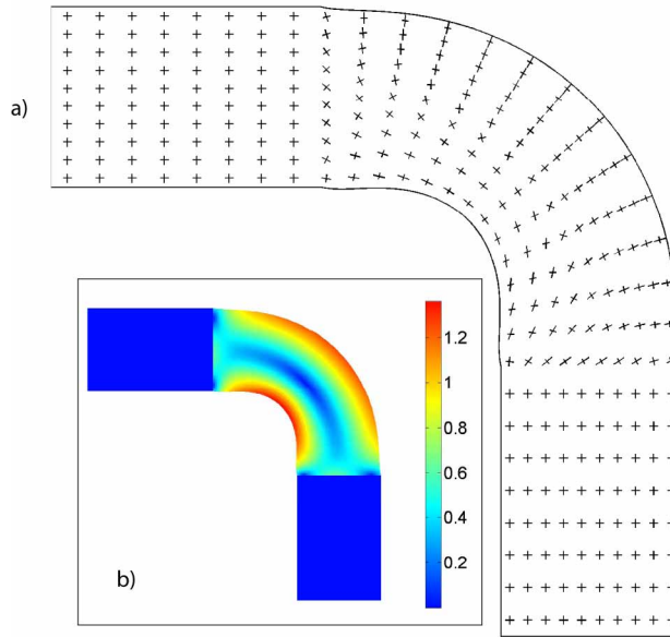
Fig. 3. Anisotropy of \varepsilon = (\eta')^{-1} illustrated with crosses oriented in the principal directions (a). The relative difference between the principal directions (b) defined as (q_1 - q_2) / (\frac{1}{2}(q_1 + q_2)) where q_i are the eigenvalues. In the straight entrance and exit of the geometry the permittivity is isotropic with a value of \varepsilon_{\text{inout}} = 3 such that the eigenvalues in \Omega satisfy 1.31 \leq q_2 \leq q_1 \leq 6.89 . The transformation is nearly incompressible and governed by Eq. (7).
