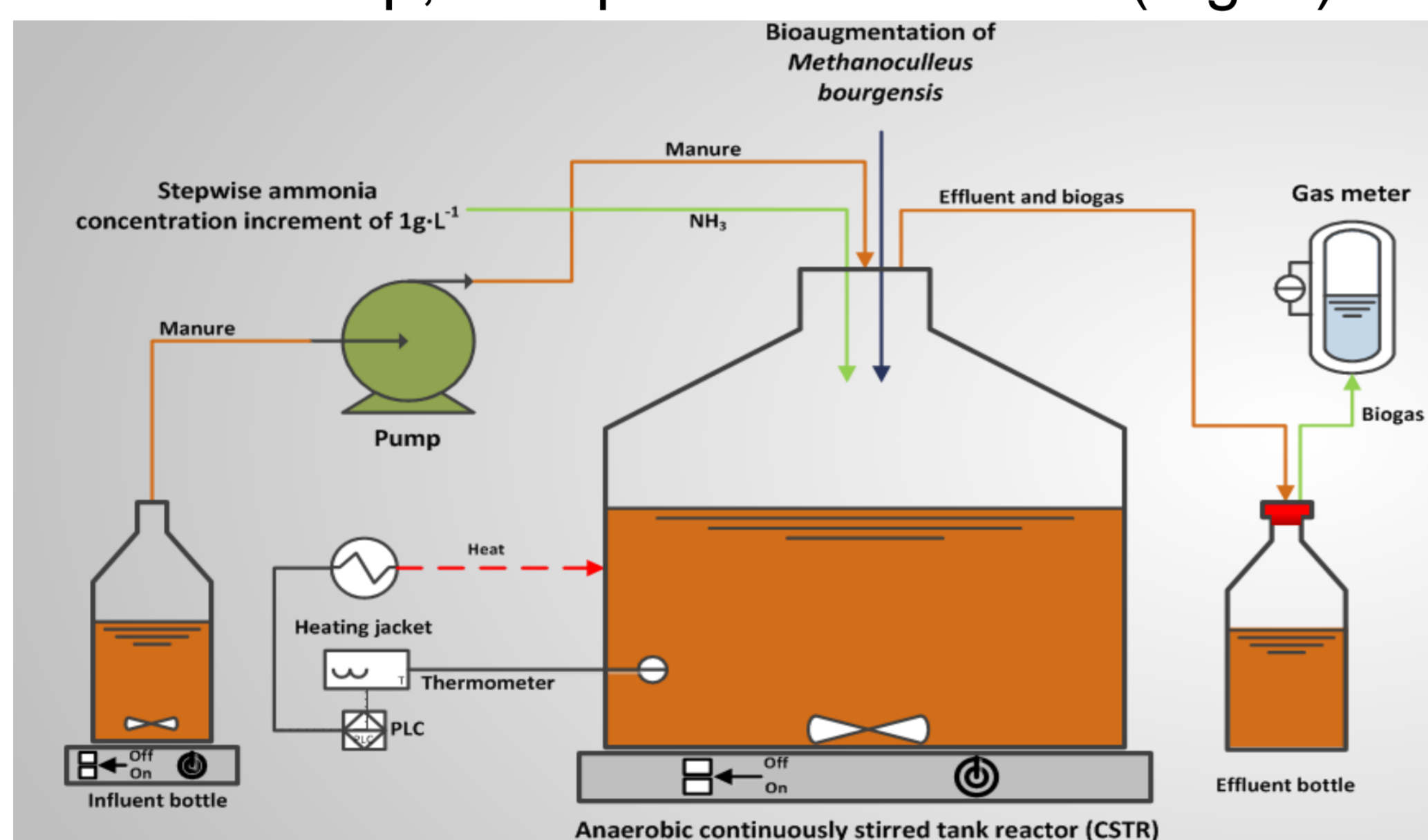
Figure 2. Experimental set-up
