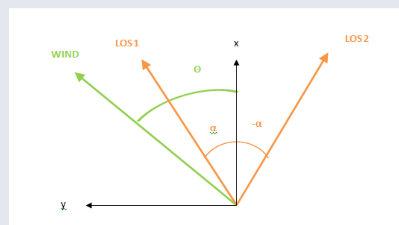
Simplified sketch showing the lidar lines of sight and the wind vector in the horizontal plane. The x-axis is aligned with the lidar axis. \alpha is the beam half-opening angle; \theta the horizontal wind direction.
