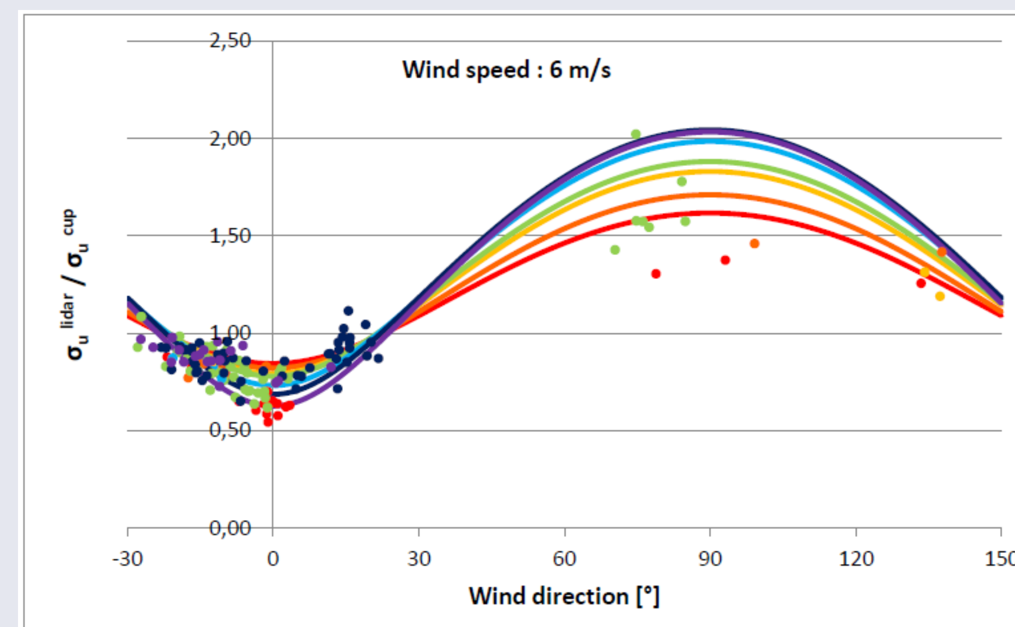
Comparison of the theoretical and experimental systematic errors for the longitudinal component of the wind speed as function of the wind direction relative to the lidar axis, for various atmospheric stability classes (different colours); for the 6 m/s wind speed bin.
