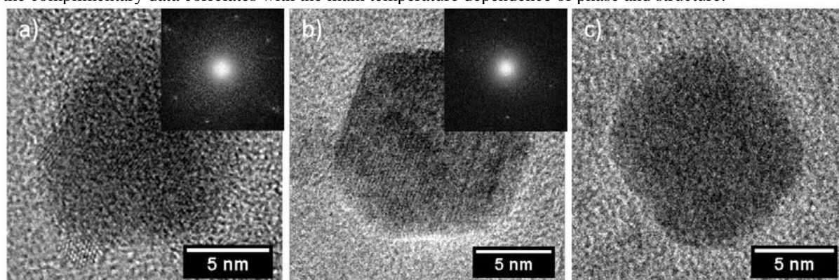
Figure 1. HRTEM and FFT of a) passivated NiGa particle at RT in vacuum, b) the reduced NiGa particle in \text{H}_2 at 350°C, and c) the NiGa particle in 75% \text{H}_2 and 25% \text{CO}_2 at 200°C.
