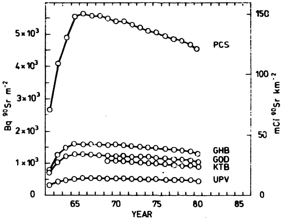
Fig. 2.1. Accumulated 90 Sr at Prins Chr. Sund, Godthåb, Godhavn, Kap Tobin and Upernavik calculated from precipitation measurements since 1952. The accumulated fallout by 1962 was estimated from the Danish data (cf. Rise Report No. 447 2 ), Appendix D) and from the ratio between the 90 Sr fallout at the Greenland stations and the fallout in Denmark in the period 1962-1974.
