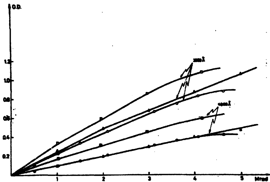
Fig. 3. Calibration curves for heat treatments of 15, 30, 60 minutes at wave-lengths 3000 Å (▲, ○, □) and 4000 Å (◆, ▼, ×).
