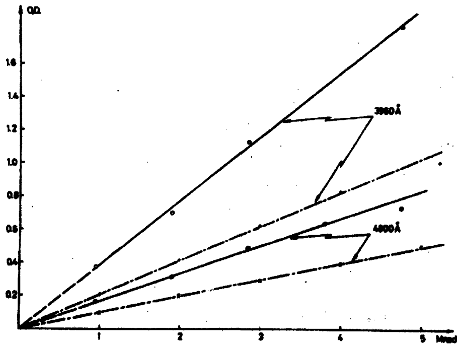
Fig. 8. Heat treatment for 35 minutes at 60°C applied to PVC films after irradiation by Co^{60} facility and electron beam. The curves are: at wave-length 3900 Å: ◦- Co^{60} , + - Aes; at 4900 Å: ◦- Co^{60} , x - Aes.
