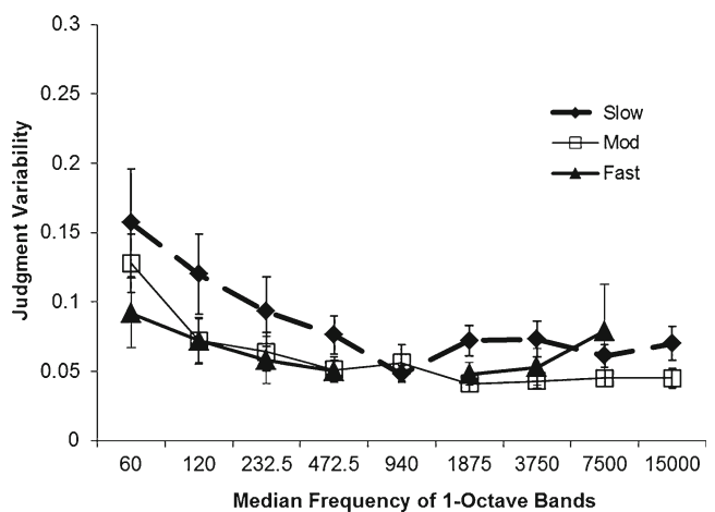
Fig. 5 Judgment variability (JV) values for the Spectral Band × Speed interaction (slow = 35.5 km/h, mod = 70 km/h, fast = 141 km/h) in Experiment 3. JV is the standard deviation of the judgments across the three iterations of each trial per participant, then averaged together for the group. Results are given with standard error bars
