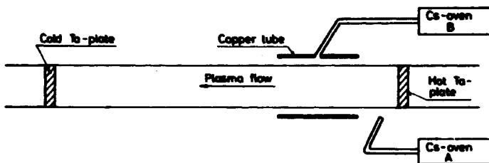
Fig. 1. Schematic of the experimental arrangement.
