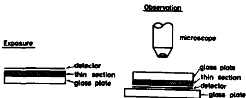
Fig. 13. Orientation of a detector-thin section sandwich for exposure and observation.
