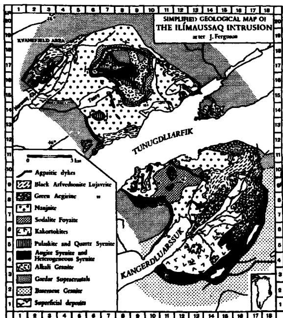
Fig. 2. Location and geologic map of the Ilímaussaġ intrusion.
