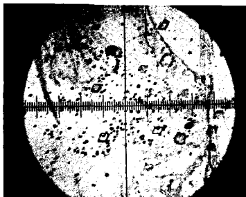
Fig. 10. Fission tracks from U plus Th (U ~ 1200 ppm, Th ~ 12000 ppm) in monazite (gray) with arfvedsonite (black), in medium to coarse lujavrite. The large tracks are from a 16-hour etch prior to the fast-neutron exposure. Field diameter 1.2 mm.
