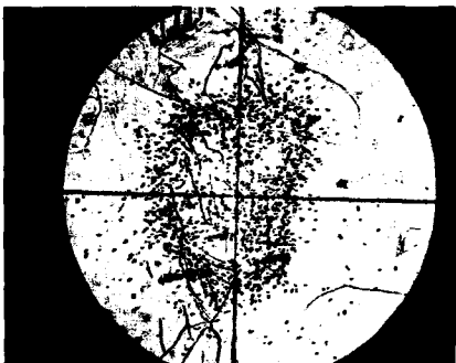
Fig. 12. Enrichment in U (2500 to 3000 ppm) at the margin of an opaque grain (hematite ?) in fluoritized fault-zone breccia, East Greenland. Field diameter 0.88 mm.
