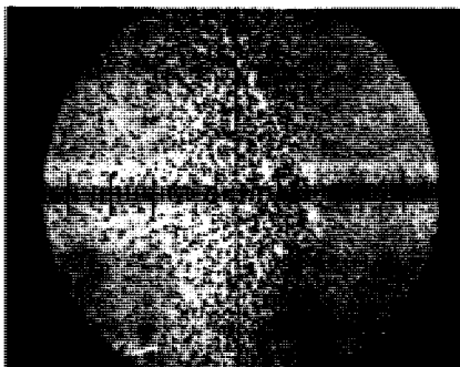
Fig. 5. Edge alteration of eudialyte in pegmatite, showing concentration of U in the rim zone (~ 7000 ppm) decreasing toward the interior of the crystal (400 ppm). Field diameter 1.2 mm.
