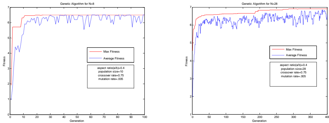
Figure 2: Variation of fitness with number of generations for N=8 and N=28
