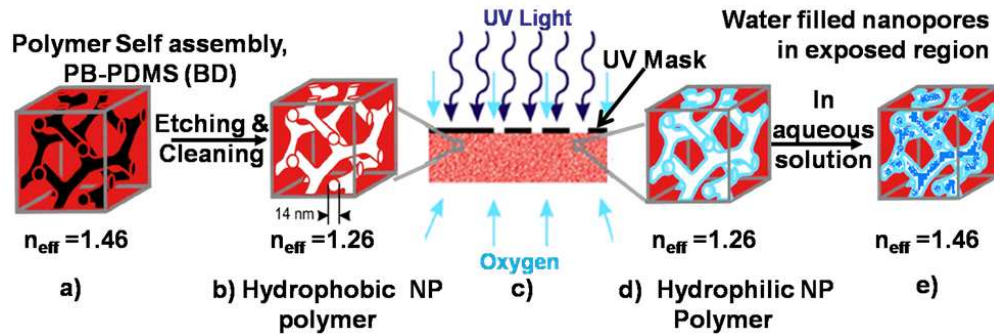
Fig. 1. Schematic illustration of working principle of Liquid Core waveguiding in n_{1,2} -PB nanoporous polymers (a) Polymer self assembly of PB-PDMS, (b) Minority block etched hydrophobic NP polymer, (c) Selectivity UV exposure using a UV mask in presence of oxygen, (d) Hydrophilic NP polymer formed at exposed regions, (e) Exposed region infiltrated with water have changed effective refractive index.
