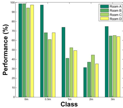
Fig. 7. Performance of the method as a function of distance for the four different rooms using speaker-independent speech model.
