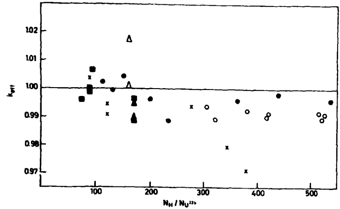
Fig 5.2.e. Calculated k_{eff} versus H to U^{235} atom ratio.
