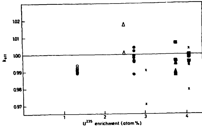
Fig. 6.2.c Calculated k_{eff} versus enrichment
