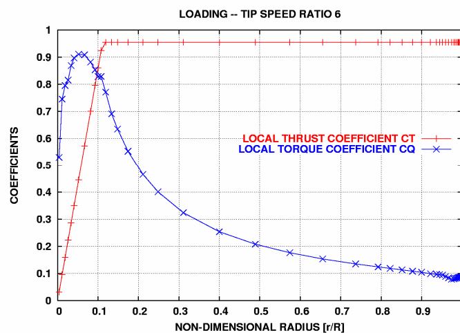
Figure 2-1 A constant thrust coefficient C_T as function of radius and the corresponding tangential loading for an ideal rotor (airfoil C_D = 0 ) at a tip speed ratio of 6.
