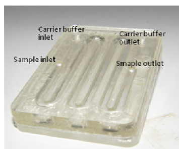
Figure 3. Sample preparation cartridge
