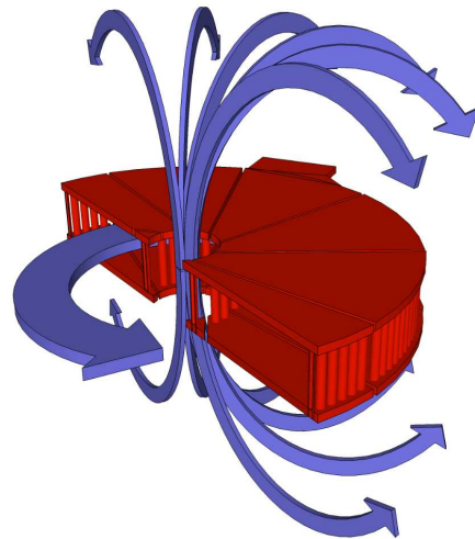
Fig. 5: PCB integrated inductor from [41]. The copper contained in the PCB is shown in red. The blue arrows mark the magnetic field.
