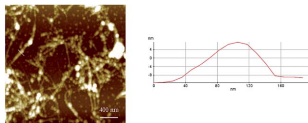
Fig. 7 Topographic image of FA-coated SWCNTs on the silicon substrate using non-contact mode imaging.
