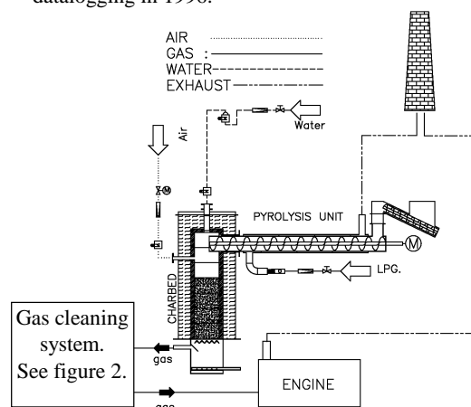
Figure 1. The 100 kW two-stage gasifier at DTU
