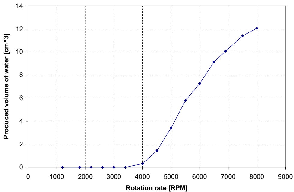
Figure F.6 Production of water vs. rotation rate for specimen 3. Total water production of 12.06 cm 3 from the pore volume of 26.84 cm 3 .
