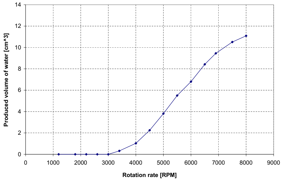
Figure F.4 Production of water vs. rotation rate for specimen 2. Total water production of 11.09 cm 3 from the pore volume of 26.55 cm 3 .
