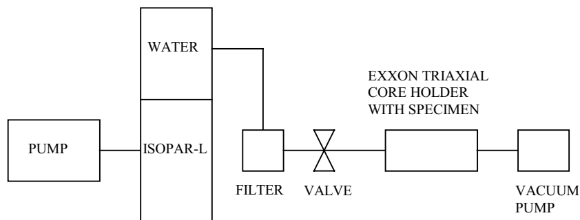
Figure 3.2 Set-up for initial fully saturation of the specimens.
