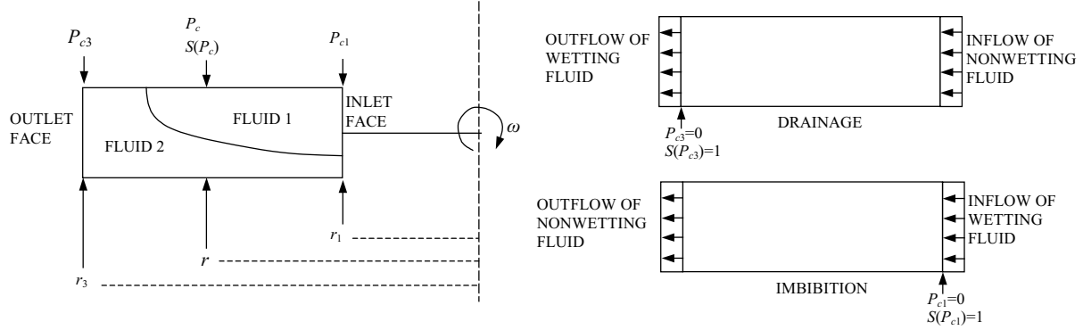
Figure 2.6 Schematic of the centrifuge method (Forbes 1994).
