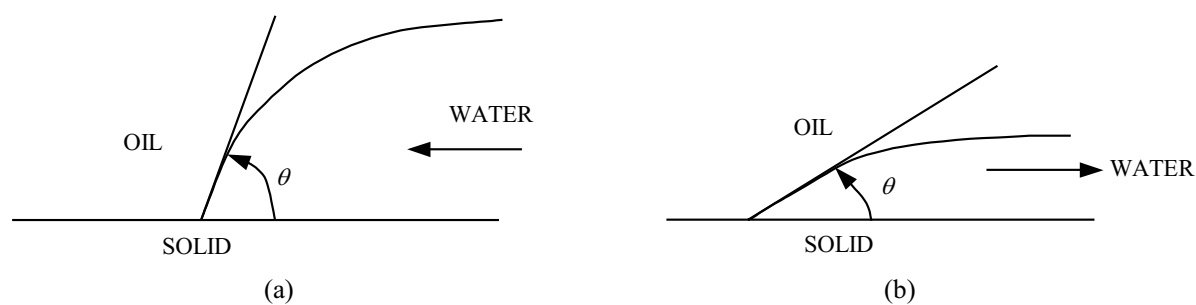
Figure 2.2 Hysteresis in contact angle in a water-wet porous medium (a) increase in the wetting fluid (imbibition) and (b) decrease in the wetting fluid (drainage).
