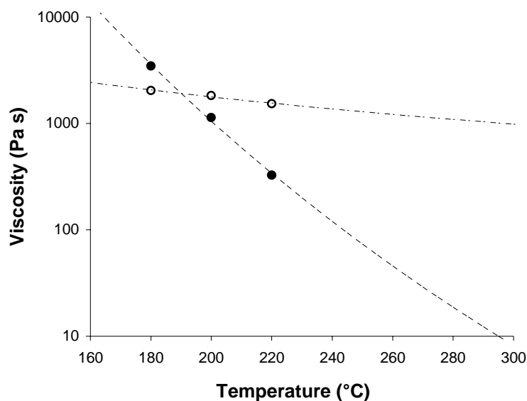
FIGURE 4.48. Viscosity as a function of temperature for PET (filled symbols) and PE (empty symbols). The dotted lines are the theoretical Arrhenius relationships calculated by equation (4.55).
