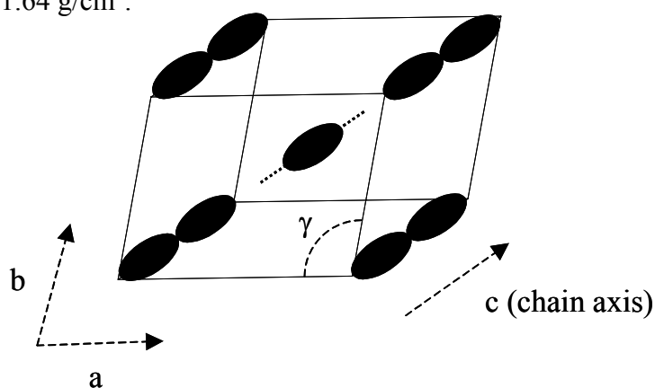
FIGURE A.2. The crystal unit cell of cellulose I \beta . The ellipses represent the glucose molecules of the cellobiose units. The two half glucose molecules in the central chain are omitted for reasons of clarity.
