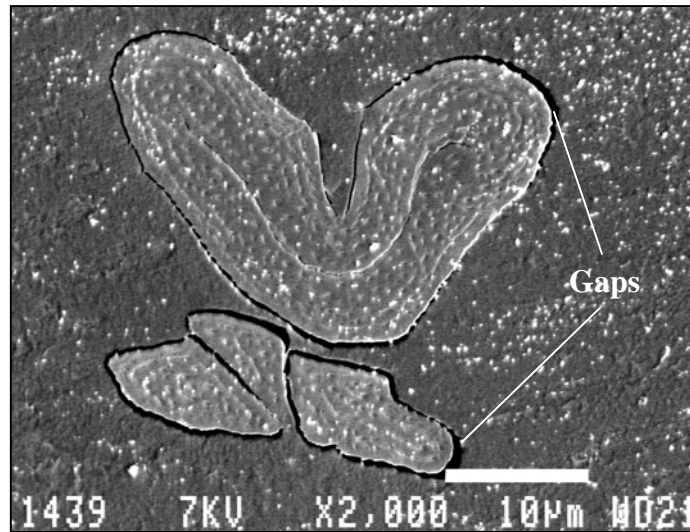
FIGURE 4.13. SEM image of four hemp yarn fibres embedded in a PP matrix. Scale bar is 10\ \mu\text{m} . The white dots are not part of the composite material, but are probably impurities induced during the polishing process.
