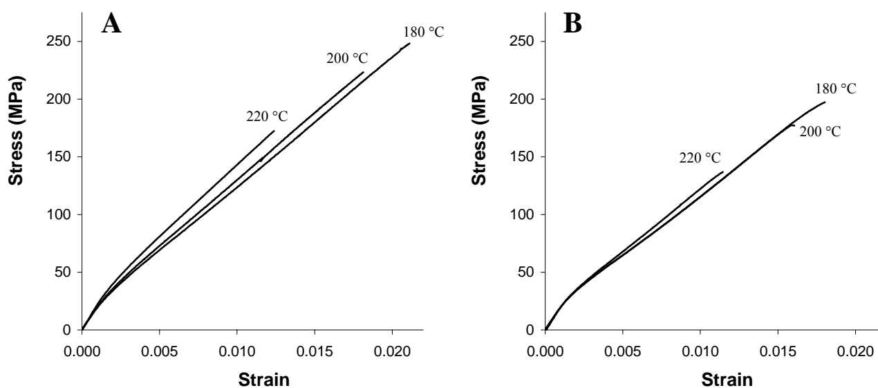
FIGURE 4.46. Representative stress-strain curves of (A) He47/PET and (B) He47/PE composites fabricated with different process temperatures. See specifications of composites in Tables 4.20 and 4.21.
