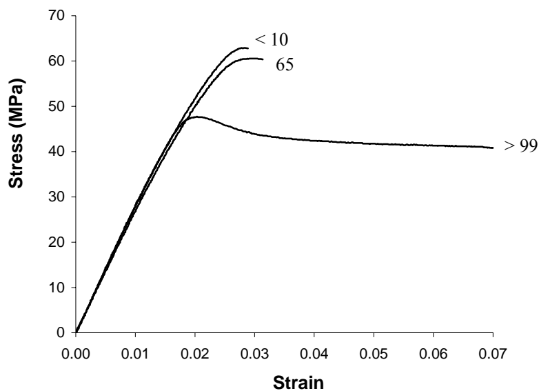
FIGURE 4.49. Representative stress-strain curves of PET conditioned at different humidities (% RH).
