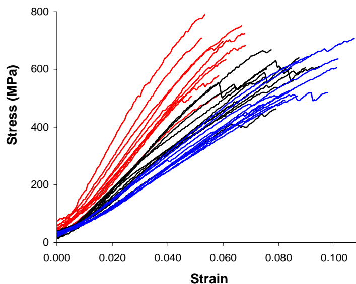
FIGURE 4.9. Stress-strain curves of He47 (red lines), He53 (black lines) and He91 (blue lines). The yarn samples were unprocessed and conditioned at 65 % RH before testing. Sample size is 10 for each yarn type.
