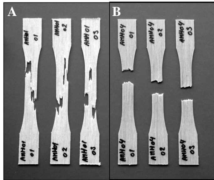
FIGURE 4.39. Failure characteristics of (A) He53/PPD D and (B) He53/MAPP tensile specimens tested in the axial direction. See specifications of composites in Table 4.17.
