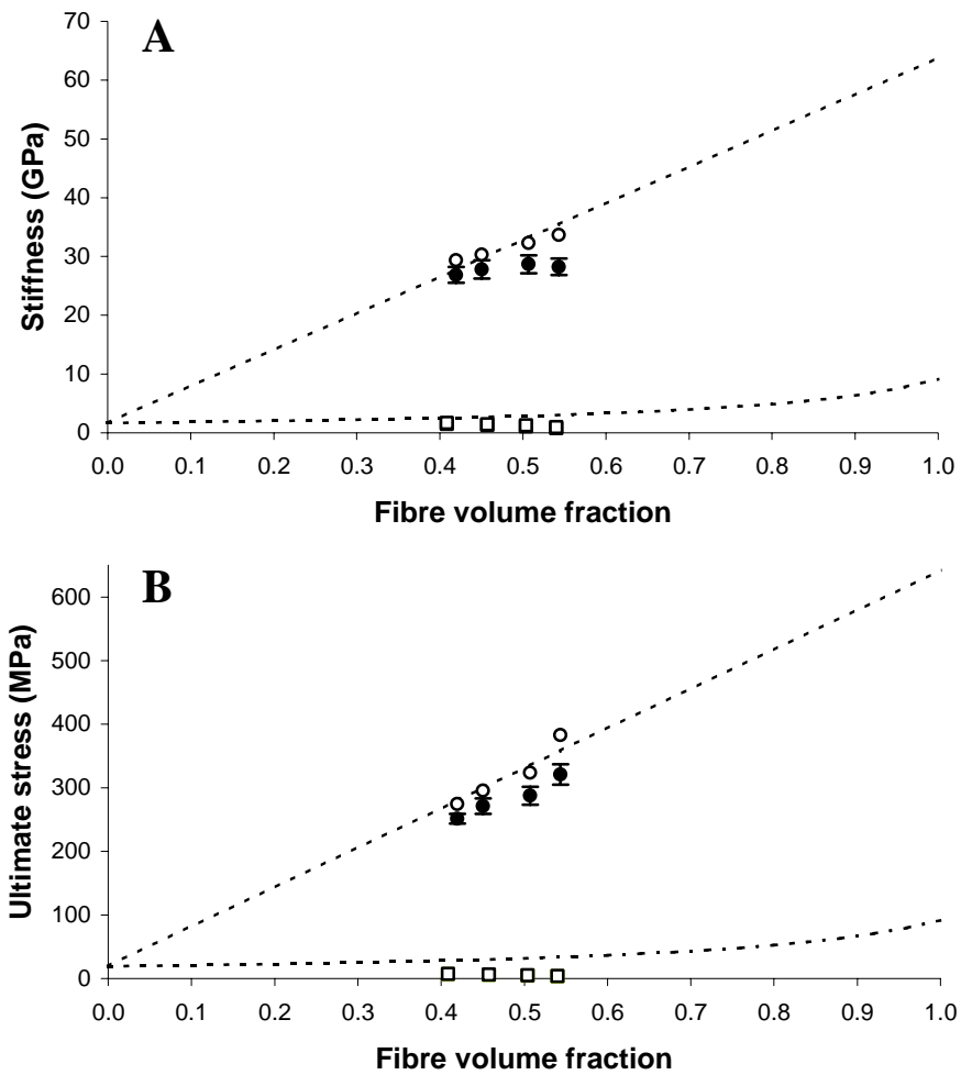
FIGURE 4.45. Tensile (A) stiffness and (B) ultimate stress of F164/PP H composites as a function of V_f . Shown are axial (o) and transverse (□) properties. Filled symbols are experimental properties and empty symbols are expected experimental properties with V_p=0 . Dotted lines are the modified “rules-of-mixtures”: equations (4.49)-(4.52) with V_p=0 . See specifications of composites in Table 4.12.
