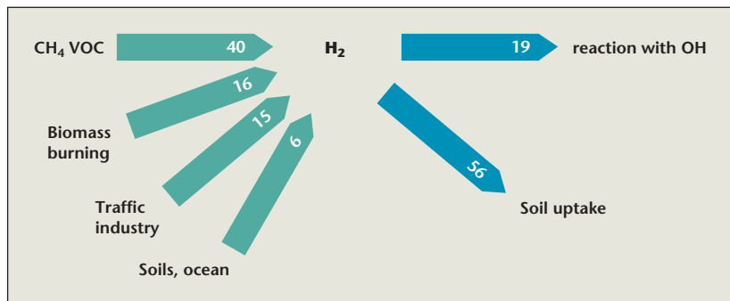
Figure 31: Sources and sinks for hydrogen in the atmosphere (million tonnes/year). The numbers are uncertain, especially for traffic and industry emissions (±10 million tonnes/year) and soil deposition (±15 million tonnes/year).
