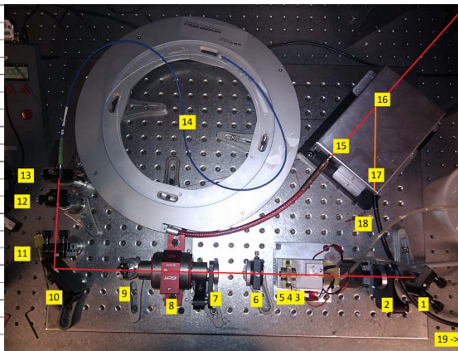
Figure 1. This is a picture of the pump laser, along with a numbered table of components. The power supplies and cooling pumps are not shown.
