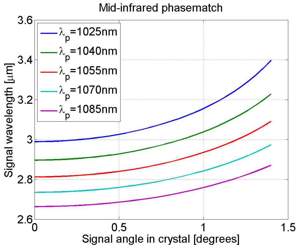
Figure 3. This picture shows the mid-IR wavelengths that are converted as function of angle through a PPLN crystal with a poling period of 20.58 μm for five different pump wavelengths.
