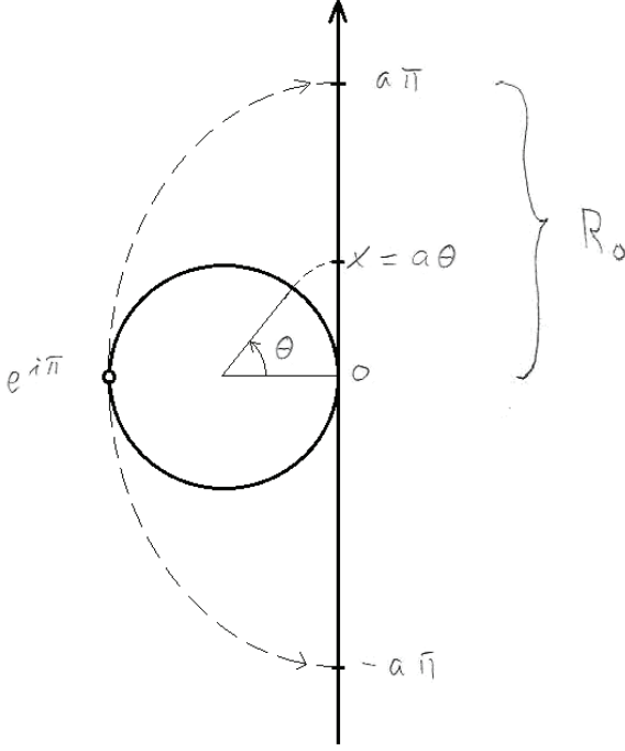
Fig. 1: Projection from configuration space to laboratory space.
