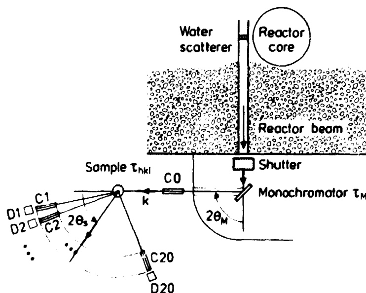
Fig. 4. The multi-detector powder diffractometer at DR 3, Risø. Twenty detectors D1...D20 with Soller collimators C1...C20 spans 100^\circ of scattering angle so a 5^\circ scan of the detector bank furnishes the complete powder pattern. C0 defines the collimation of the incident beam.
