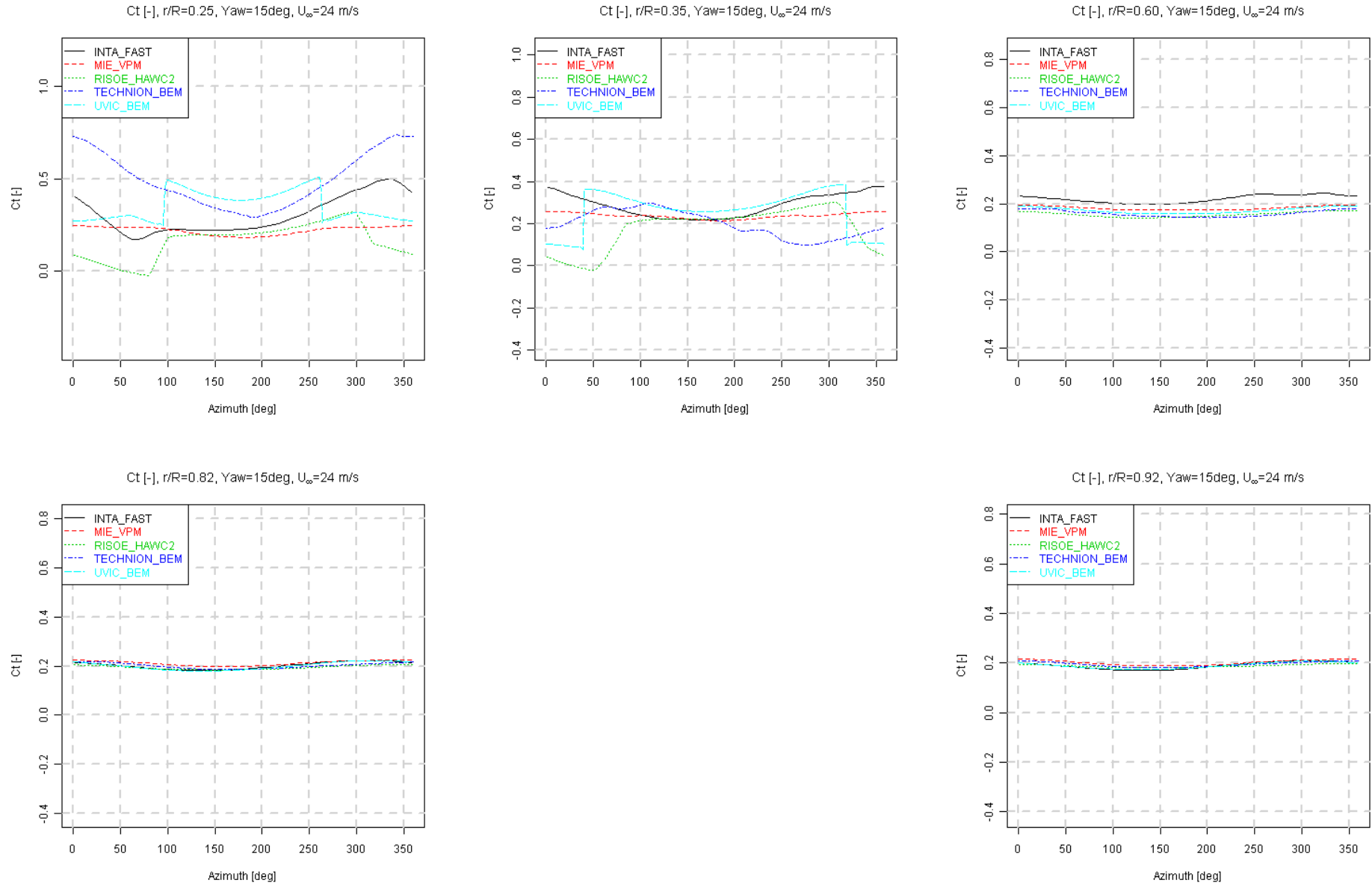
Figure 8.51 Tangential force coefficient variation with azimuth angle, U_\infty = 24 m/s, \text{Yaw} = 15^\circ
