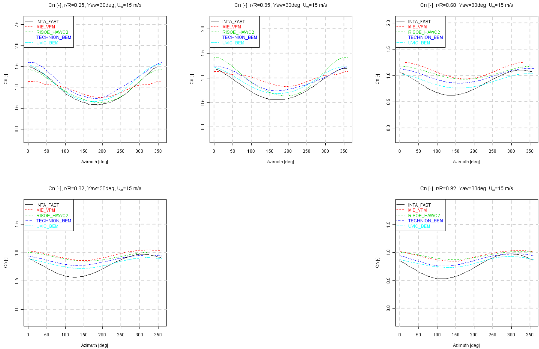
Figure 8.44 Normal force coefficient variation with azimuth angle, U_\infty = 15 m/s, Yaw = 30^\circ
