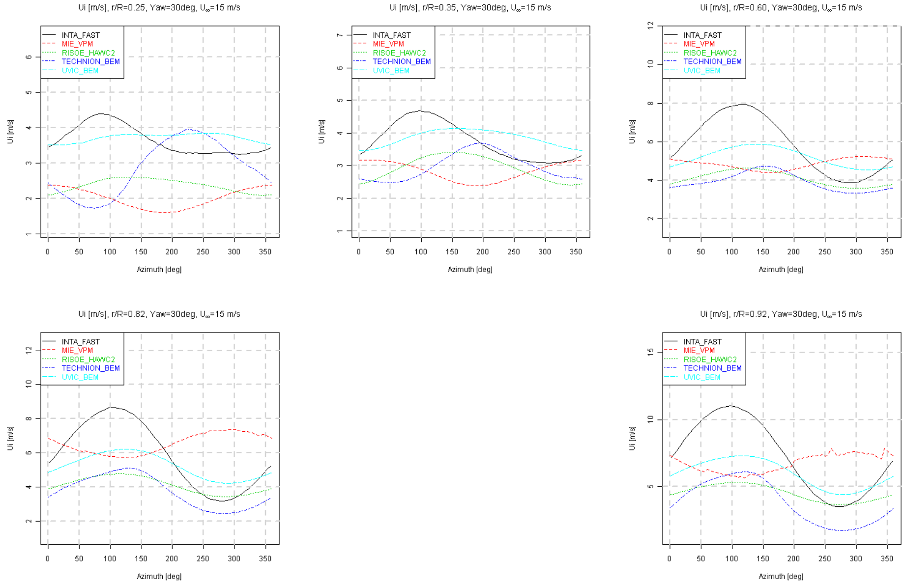
Figure 8.46 Axial induced velocity variation with azimuth angle, U_\infty = 15 m/s, \text{Yaw} = 30^\circ
