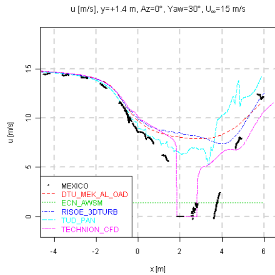
Figure 8.54 Axial traverse of velocity in x -direction, Yaw=30^\circ , U_\infty=15 m/s
