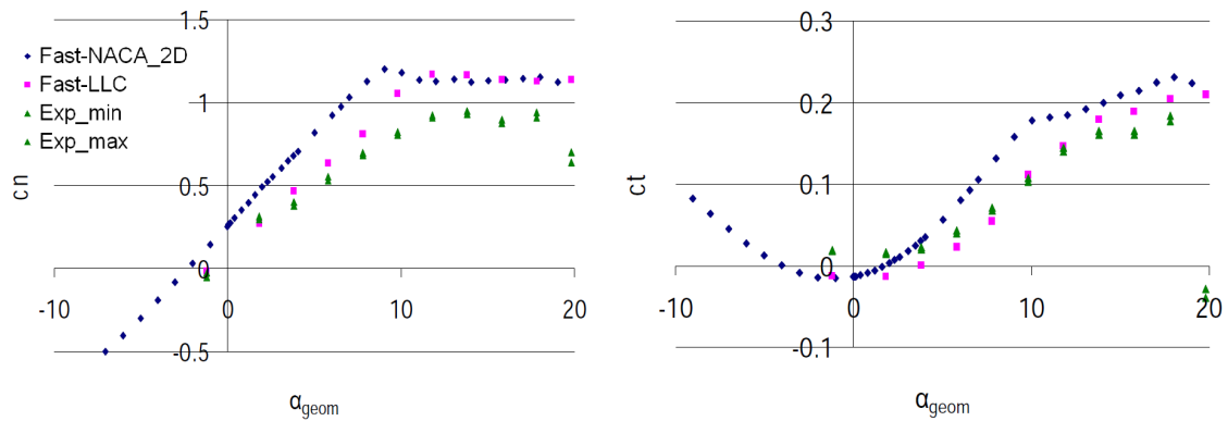
Figure 9.8 cn-\alpha_{geom} and ct-\alpha_{geom} at 92% radius (NACA 64-418)
