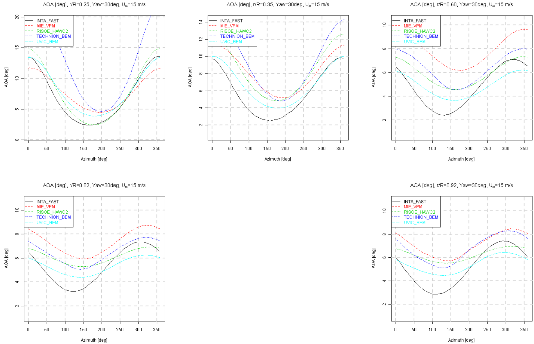
Figure 8.42 Angle of attack variation with azimuth angle, U_\infty = 15 m/s, \text{Yaw} = 30^\circ
