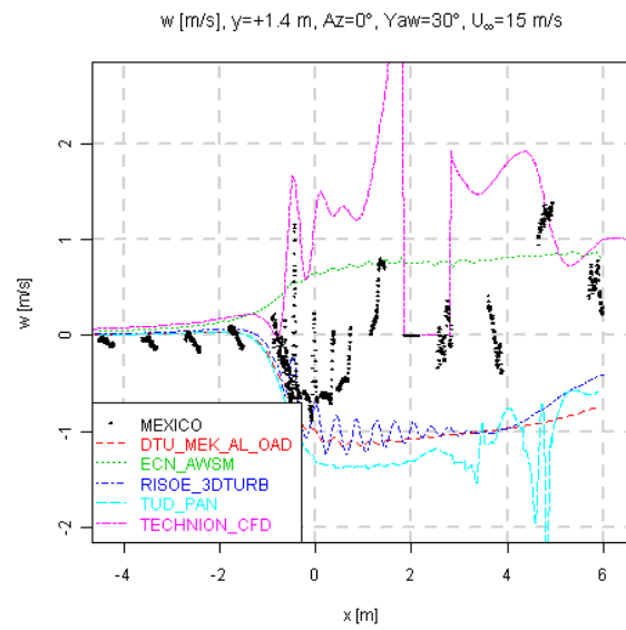
Figure 8.56 Axial traverse of velocity in z -direction, Yaw=30°, U_\infty=15 m/s
