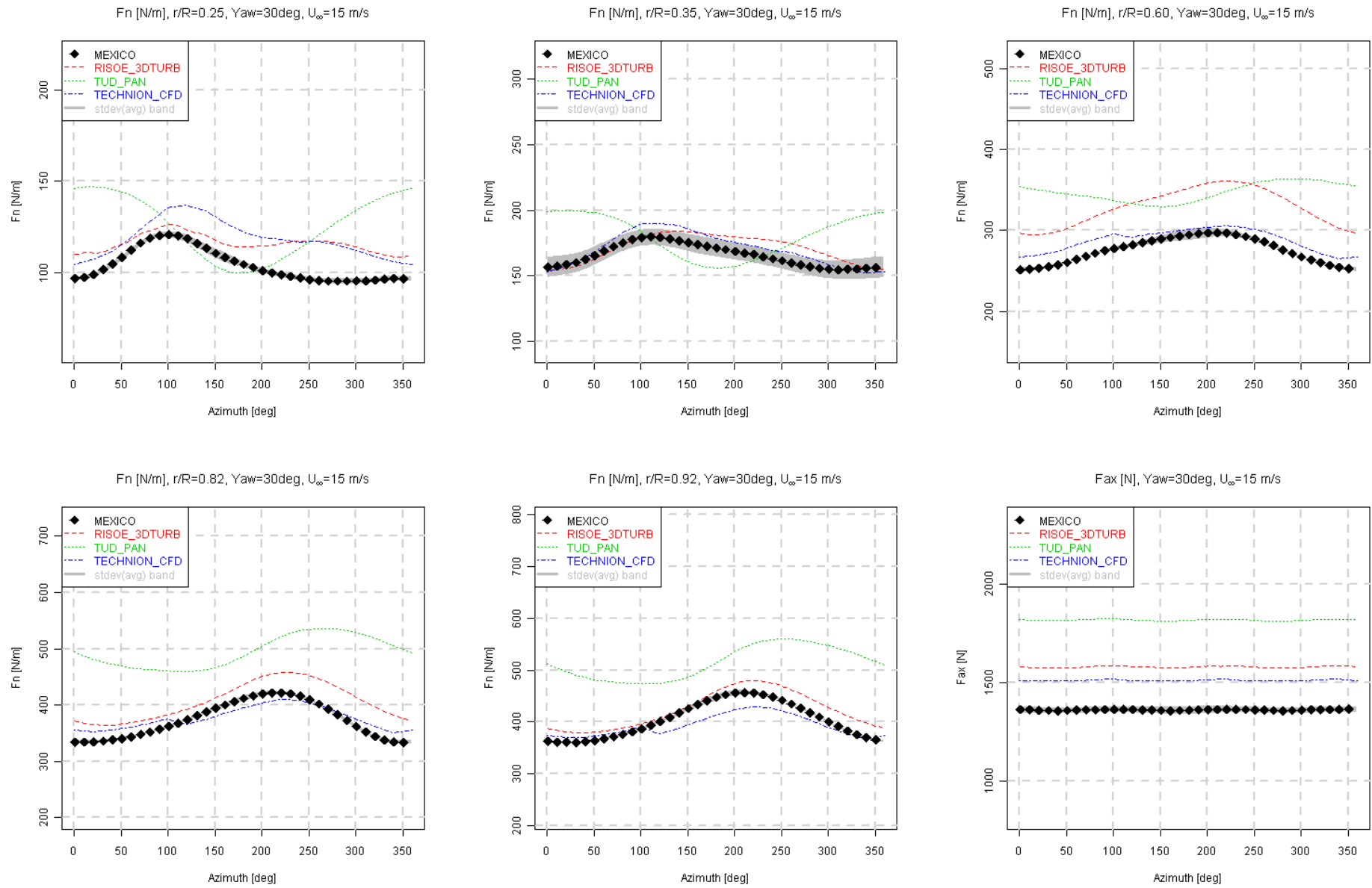
Figure 8.34 Normal and axial force variation with azimuth angle (CFD), U_\infty = 15 m/s, \text{Yaw} = 30^\circ
