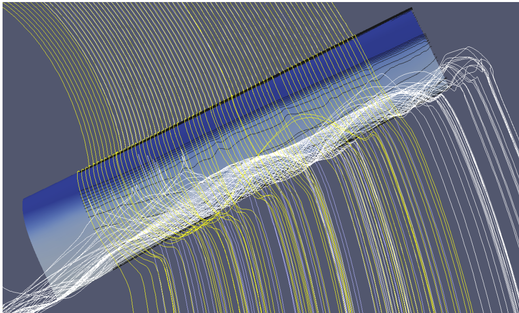
Figure 14.6 The streamlines like in fig. 14.5 expanded to a region from 0.4R to 0.65R showing that the interaction of the main stream from the tip with the 3D stall vortex is a local phenomenon
