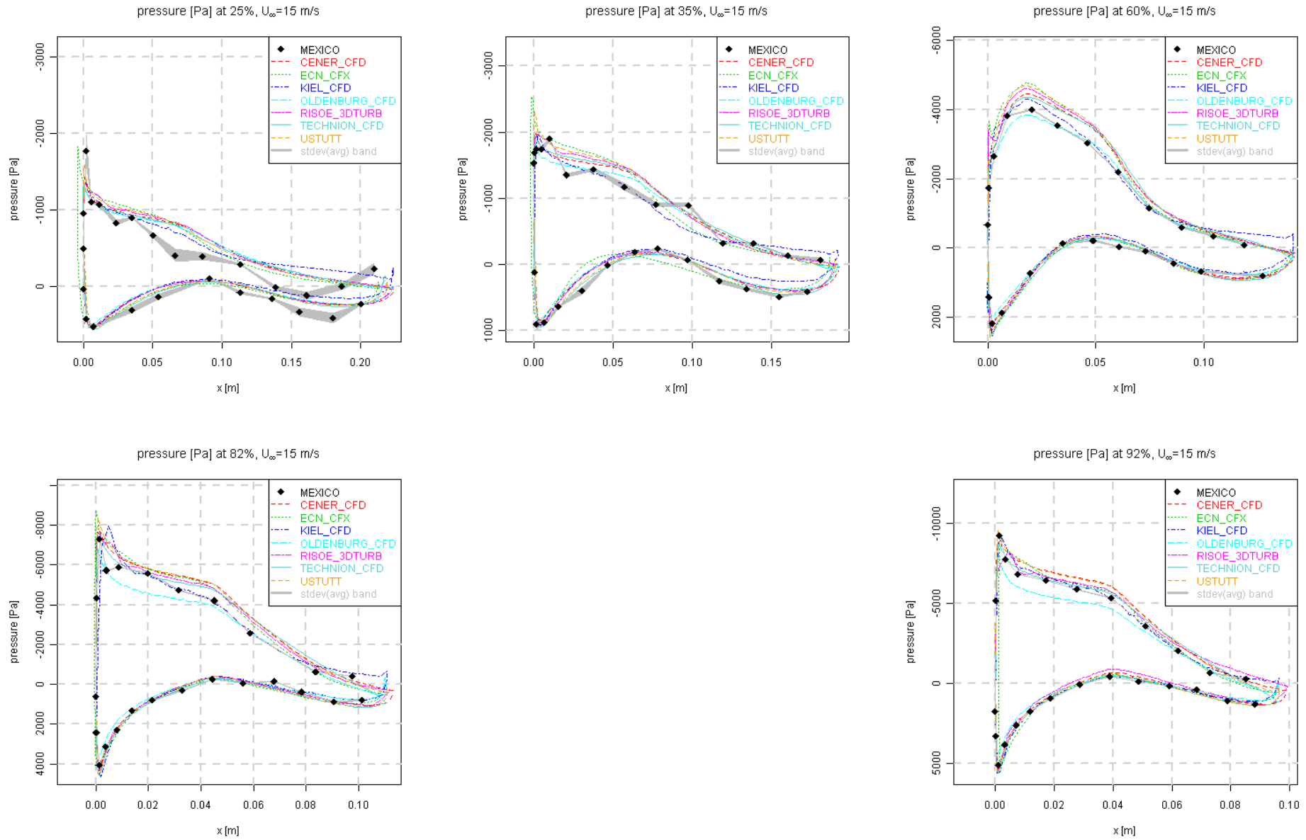
Figure 8.2 Pressure distributions for U_\infty = 15 m/s
