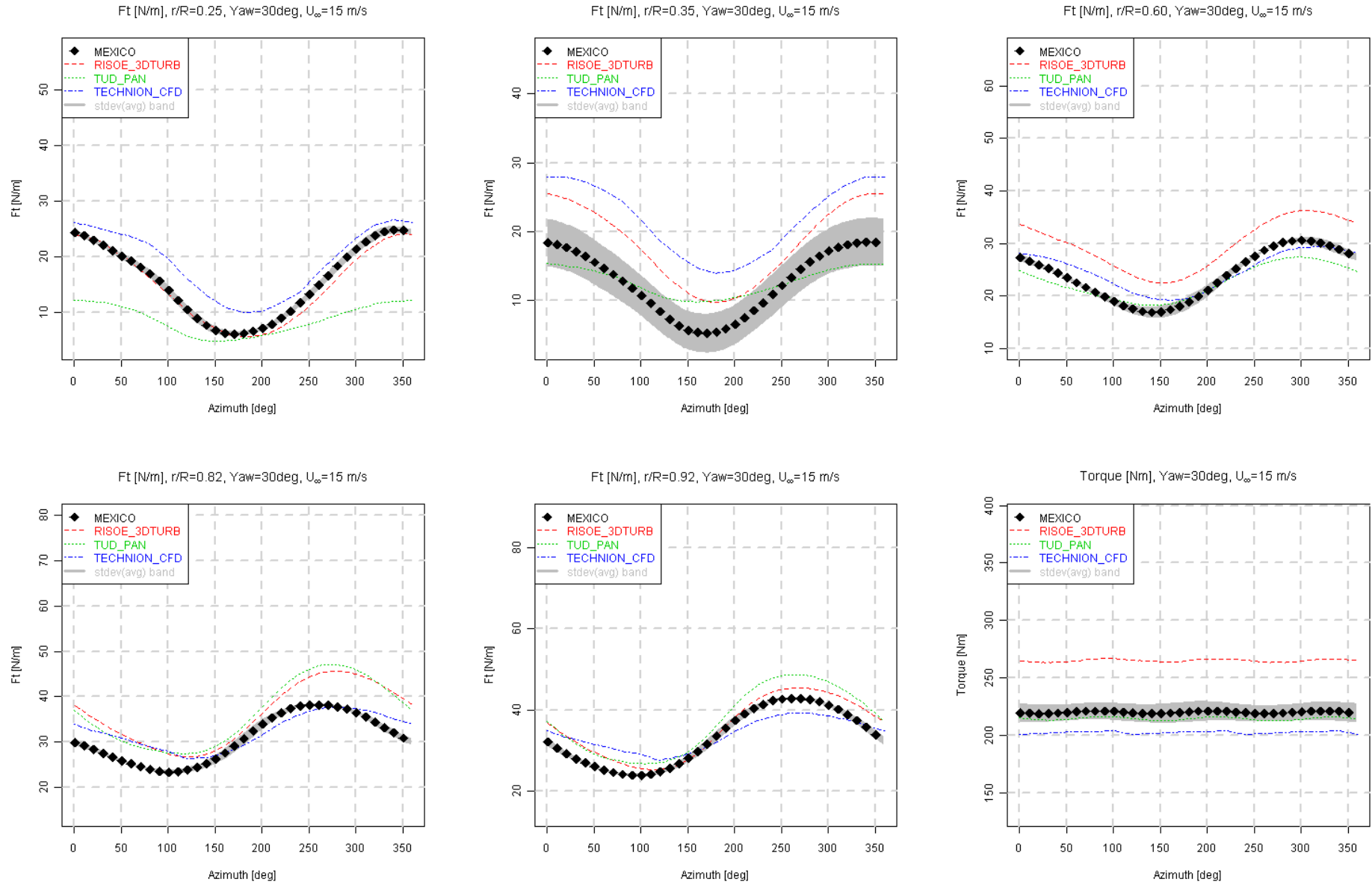
Figure 8.36 Tangential force and torque variation with azimuth angle (CFD), U_\infty = 15 m/s, \text{Yaw} = 30^\circ
