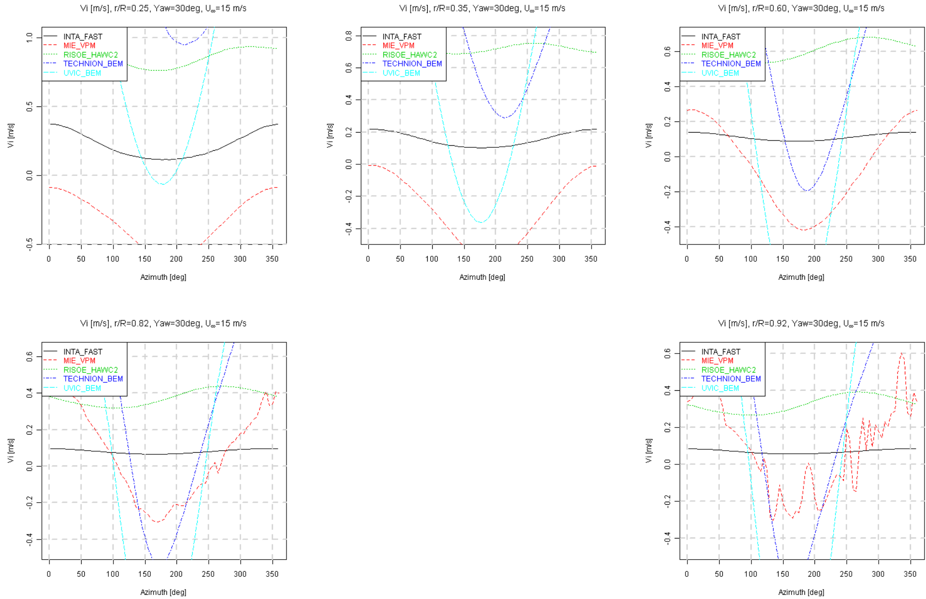
Figure 8.47 Tangential induced velocity variation with azimuth angle, U_\infty=15 m/s, \text{Yaw}=30^\circ
