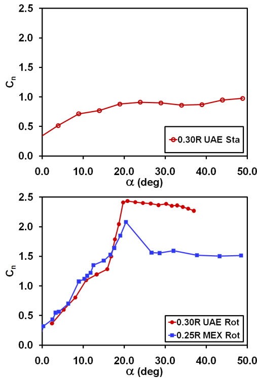
Figure 15.11 MEXICO and UAE Phase VI mean C_n at inboard radius, for parked (upper panel) and rotating (lower panel) blades.
