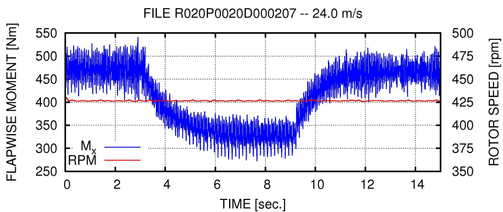
Figure 16.2 The flapwise bending moments for a pitch step from -2.3^\circ to 5^\circ and a rotor speed of 425 rpm.
