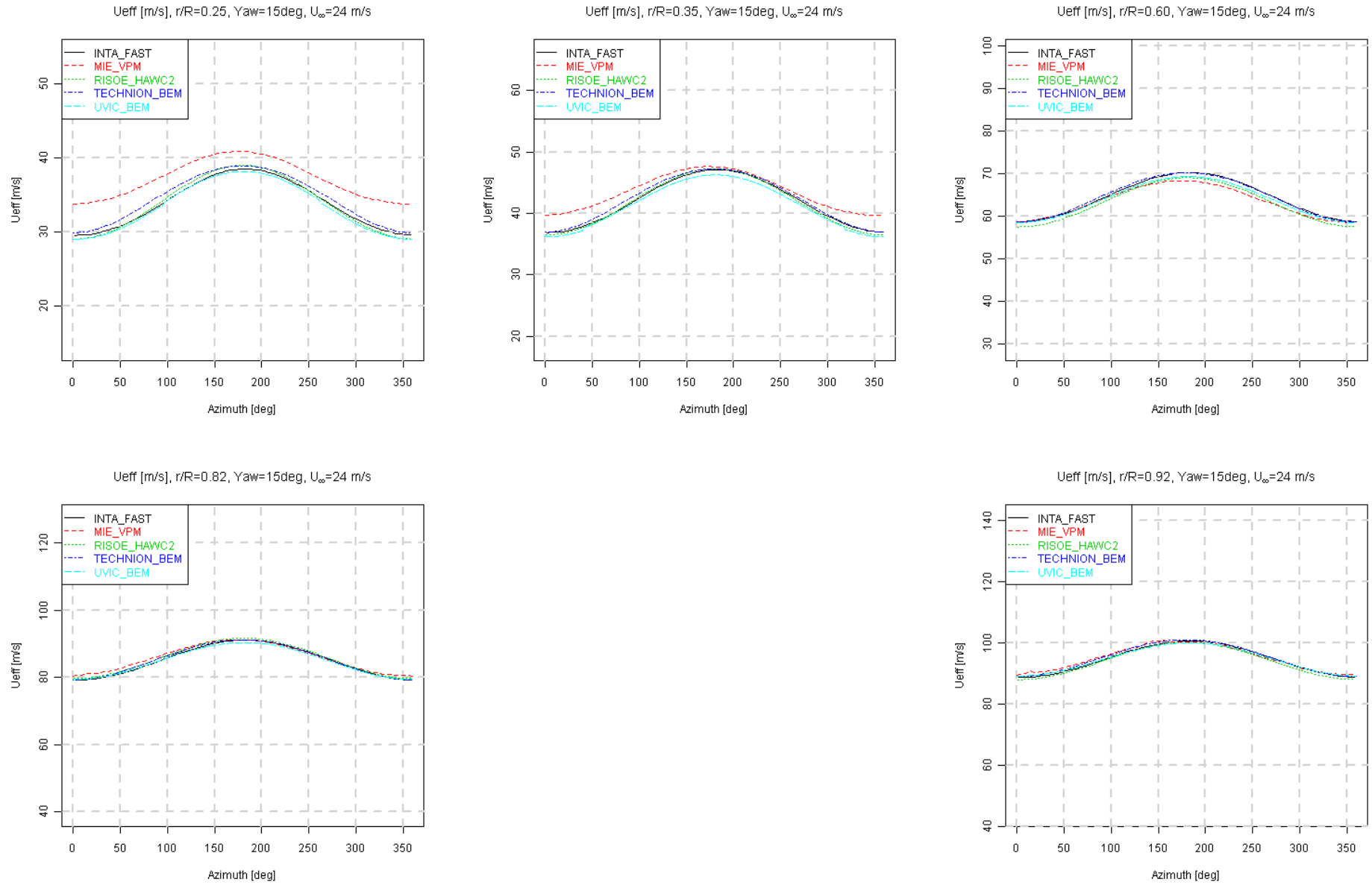
Figure 8.49 Effective velocity variation with azimuth angle, U_\infty = 24 m/s, \text{Yaw} = 15^\circ
