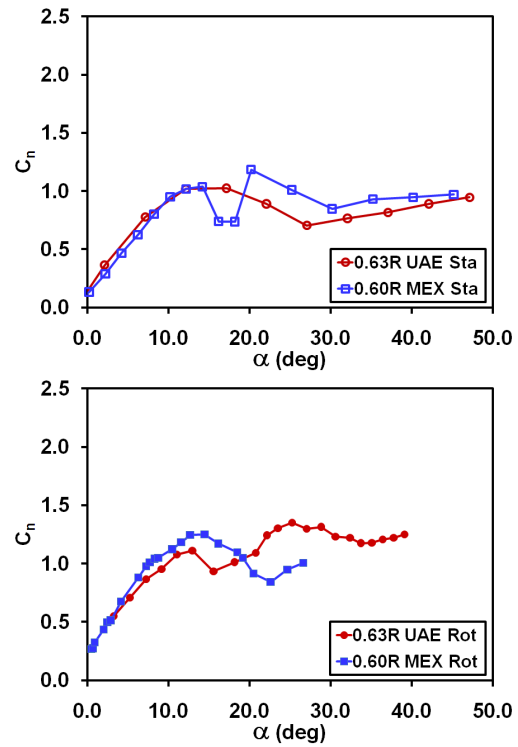
Figure 15.12 MEXICO and UAE Phase VI mean C_n at mid-span radius, for parked (upper panel) and rotating (lower panel) blades.
