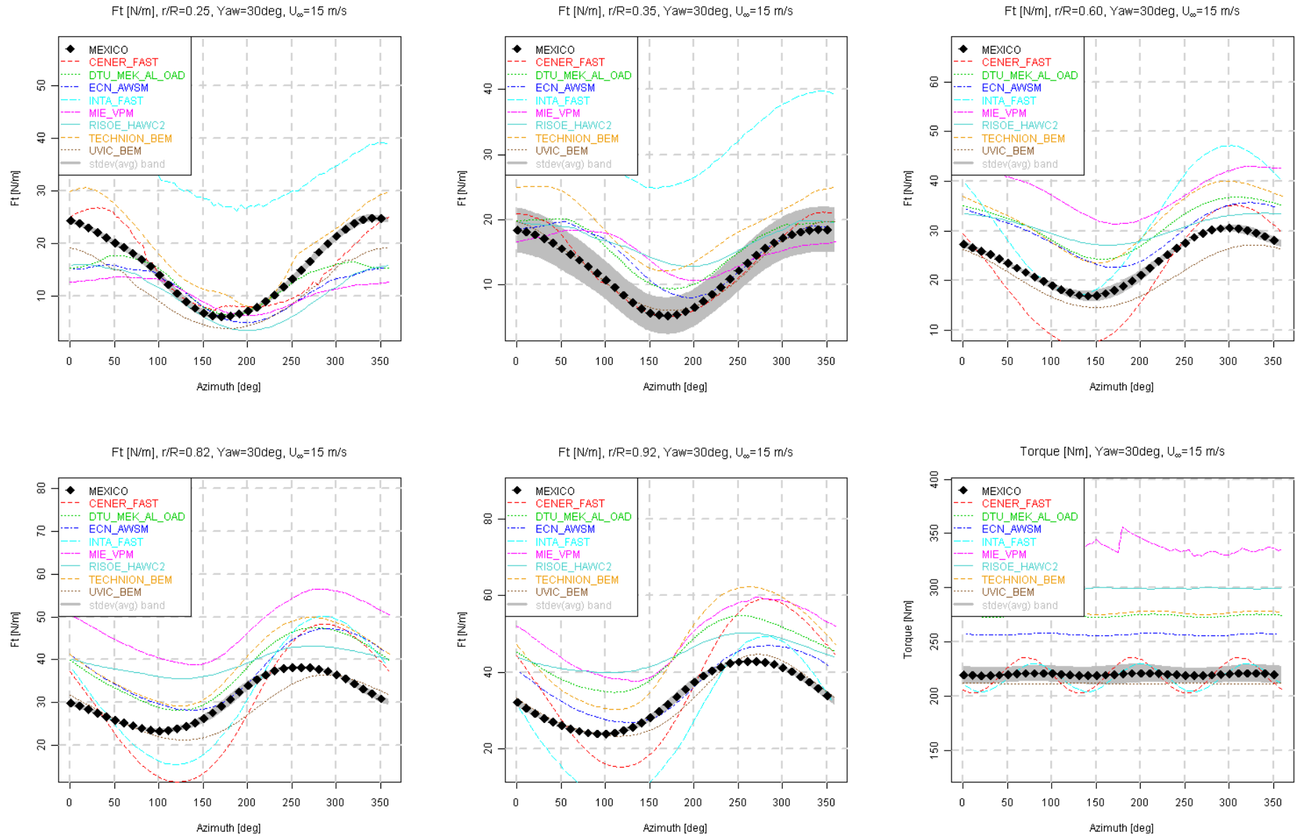
Figure 8.37 Tangential force and torque variation with azimuth angle (lifting line codes), U_\infty = 15 m/s, Yaw = 30^\circ
