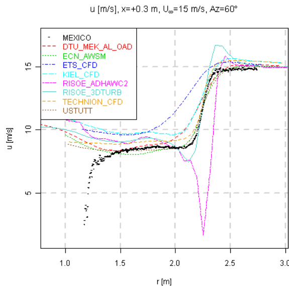
Figure 13.1 Radial velocity traverse, 30 cm downstream of the rotor, measured and calculated with CFD codes. V_{tun} = 15\text{m/s} , \Phi_r = 60 degrees
