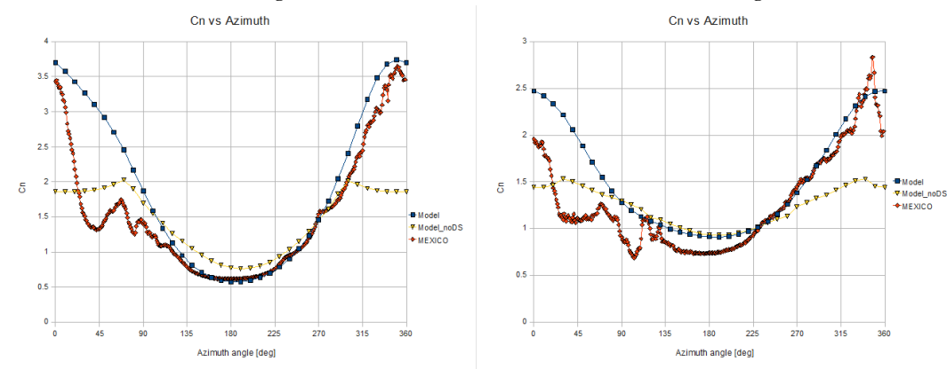
Figure 15.5 25% Spanwise Station, Figure 15.6 35% Spanwise station, \beta = 45 deg
