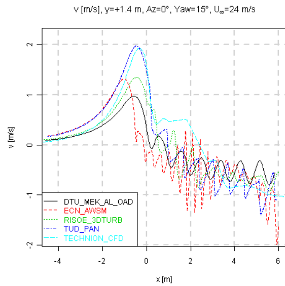
Figure 8.58 Axial traverse of velocity in y -direction, Yaw=15^\circ , U_\infty=24 m/s
