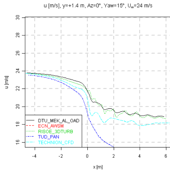
Figure 8.57 Axial traverse of velocity in x -direction, Yaw=15^\circ , U_\infty=24 m/s
