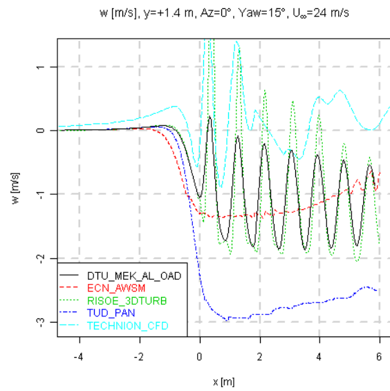
Figure 8.59 Axial traverse of velocity in z -direction, Yaw=15^\circ , U_\infty=24 m/s
