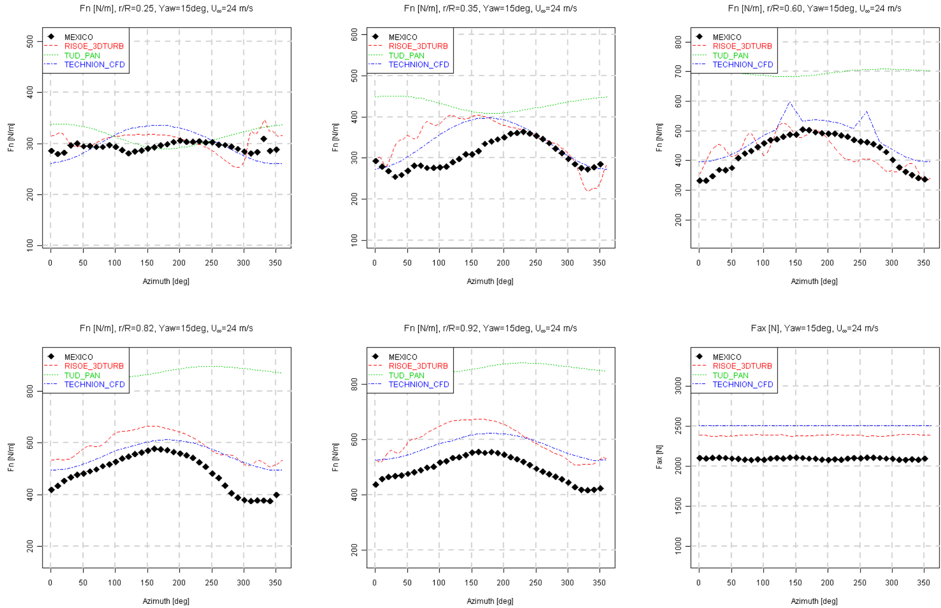
Figure 8.38 Normal and axial force variation with azimuth angle (CFD), U_\infty = 24 m/s, Yaw = 15^\circ
