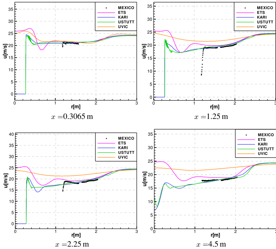
Figure 12.3 Radial traverse for 24 m/s upstream velocity at x = 0.3065 m; 1.25 m; 2.25 m and 4.5 m axial position for 0^\circ azimuth of blade one
