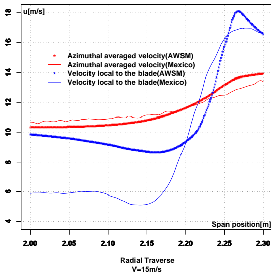
Figure 13.12 Local and azimuthally averaged velocities in the rotor plane, measured and AWSM calculated, V = 15 \text{ m/s}
