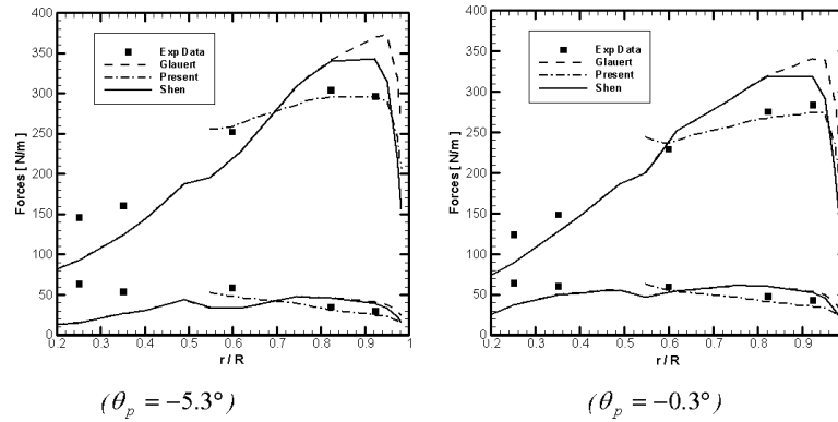
Figure 11.5 Comparison of axial and tangential force distributions determined from experimental data, BEM using derived airfoil data, BEM using 2D airfoil data for the Mexico rotor at V_0 = 16.9 m/s ( \lambda = 4.53 ) and 324.5 rpm
