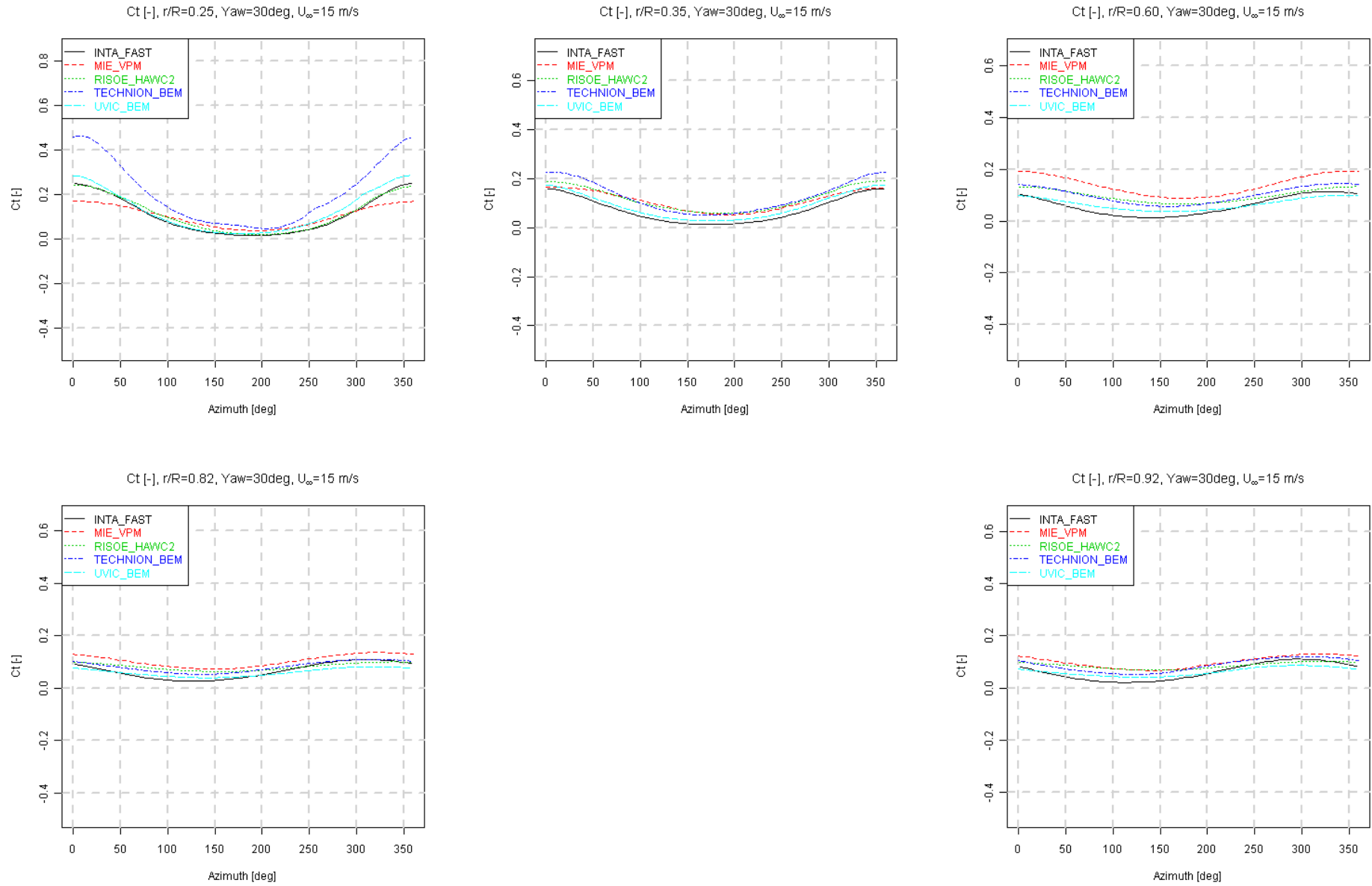
Figure 8.45 Tangential force coefficient variation with azimuth angle, U_\infty = 15 m/s, \text{Yaw} = 30^\circ
