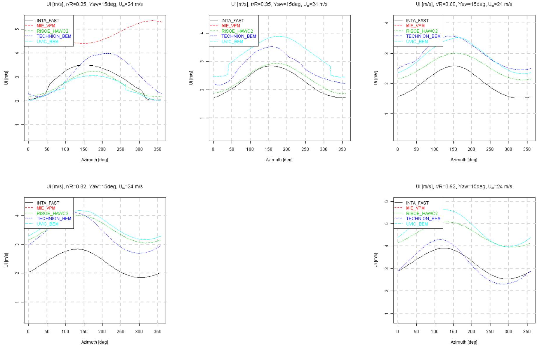
Figure 8.52 Axial induced velocity variation with azimuth angle, U_\infty = 24 m/s, Yaw = 15^\circ
