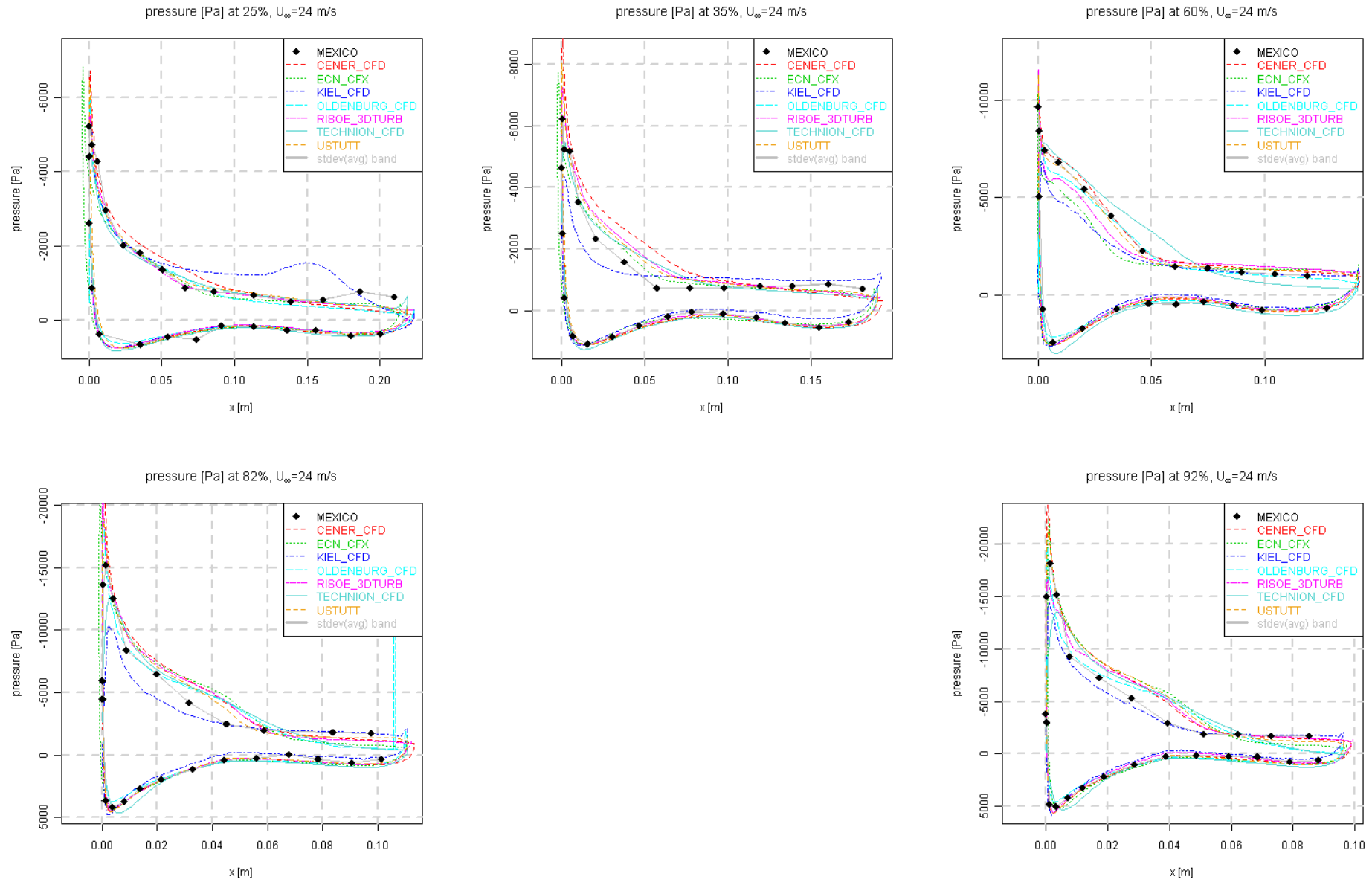
Figure 8.4 Pressure distributions for U_\infty = 24 m/s
