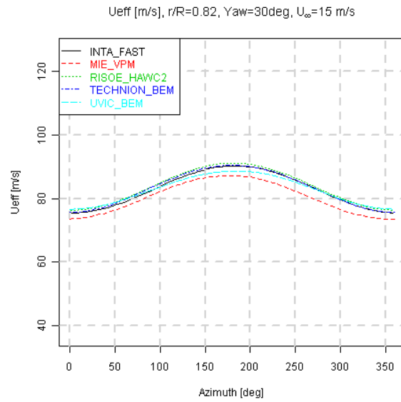
Figure 8.43 Effective velocity variation with azimuth angle, U_{\infty}=15 m/s, \text{Yaw}=30^{\circ}
