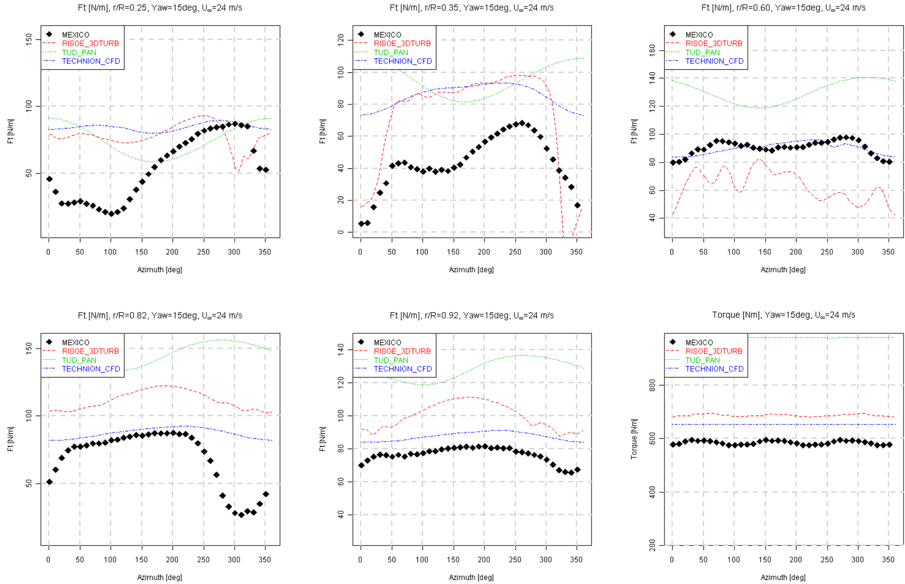
Figure 8.40 Tangential force and torque variation with azimuth angle (CFD), U_\infty = 24 m/s, Yaw=15°
