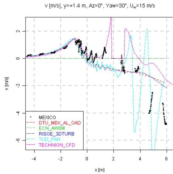
Figure 8.55 Axial traverse of velocity in y -direction, Yaw=30^\circ , U_\infty=15 m/s
