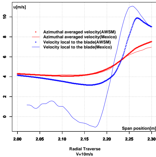
Figure 13.11 Local and azimuthally averaged velocities in the rotor plane, measured and AWSM calculated, V = 10 \text{ m/s}
