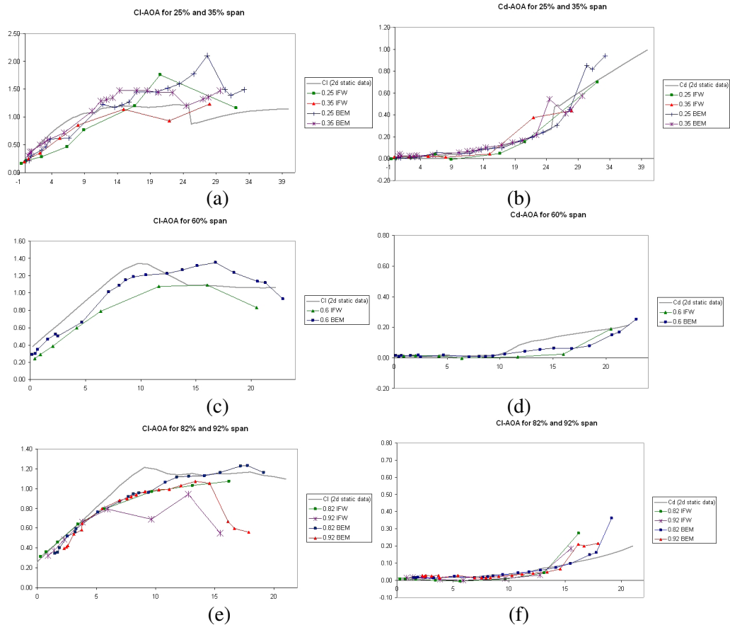
Figure 11.1 Cl and Cd versus angle of attack for the Mexico rotor at a rotor speed of 324.5 rpm and a pitch angle of -2.3 degrees, (a) Cl-α at 25% and 35% span (b) Cd-α at 25% and 35% span, (c) Cl-α at 60% span, (d) CD-α at 60% span, (e) CL-α at 82% and 92% span, (f) CD-α at 82% and 92% span
