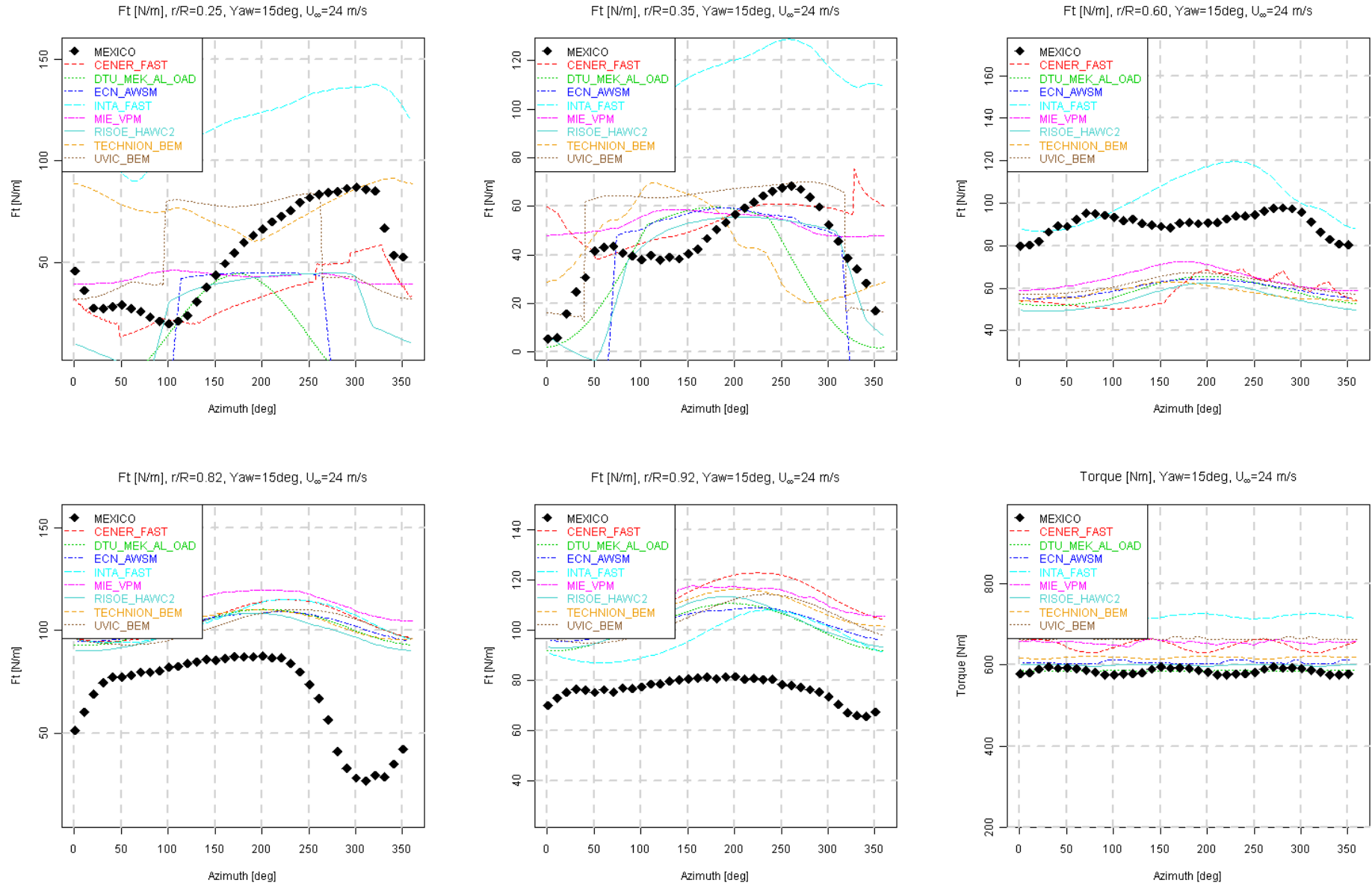
Figure 8.41 Tangential force and torque variation with azimuth angle (lifting line codes), U_\infty = 24 m/s, \text{Yaw} = 15^\circ
