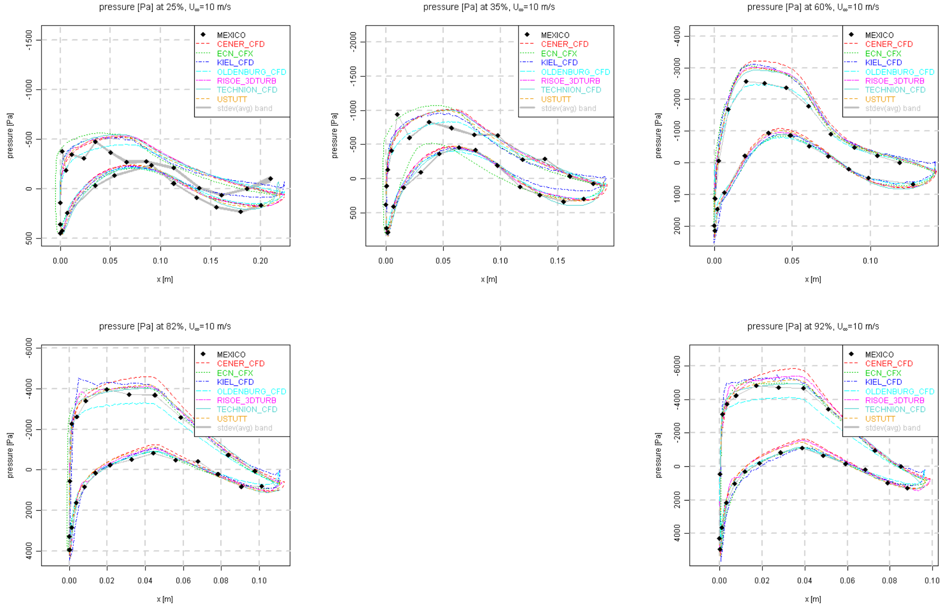
Figure 8.3 Pressure distributions for U_\infty = 10 m/s
