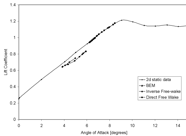
Figure 11.6 Cl - \alpha data at 92% span obtained with the inverse free wake model for the Mexico rotor at a wind speed of 15 m/s ( \lambda = 6.67 ), a pitch angle of -2.3 degrees and a rotor speed of 424 rpm
