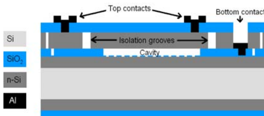
Figure 2. Schematic of the sensor layers.
