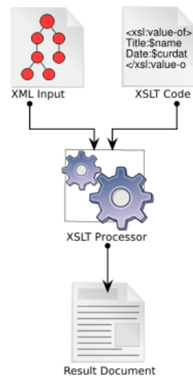
Fig. 5. Showing the transformation flow [15]
