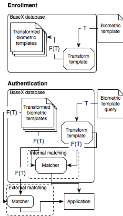
Fig. 3. Enrollment and authentication phases after implementing XCBF with feature transformation in BaseX
