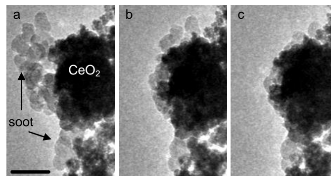
Figure 1. A time-lapsed ETEM image series of soot in contact with a CeO 2 catalyst acquired during the exposure to 2mbar O 2 at 550°C. The time interval between the images is ~2min. Scale bar, 90nm. The figure is adapted from (7).
