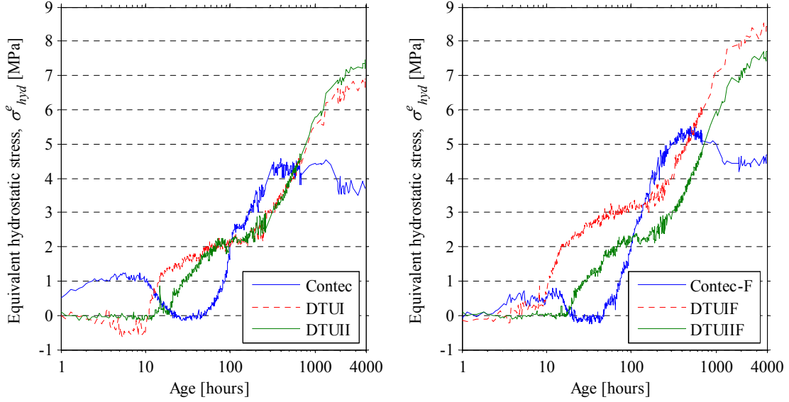
Figure 2: Development in equivalent hydrostatic stress \sigma_{hyd}^e , in the pressure sensors.
