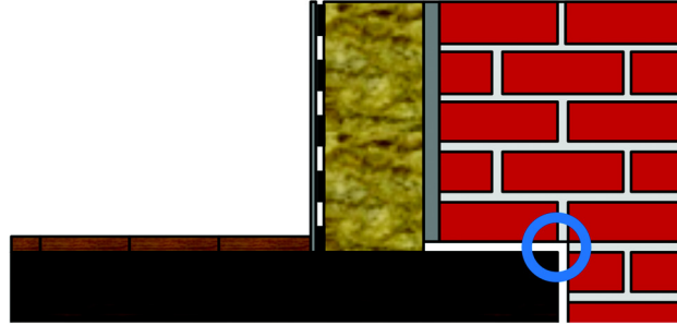
Figure 4 Wall section analyzed by hygrothermal simulation. The blue circle indicates the point of evaluated relative humidity and moisture content.
