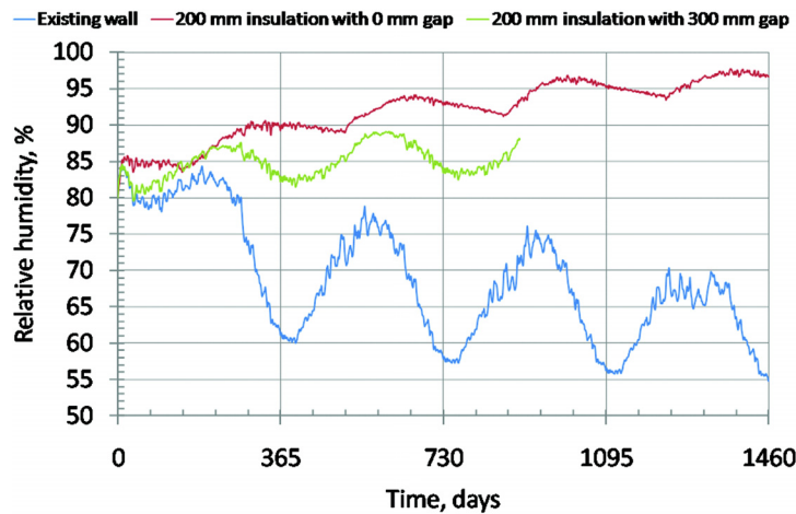
Figure 5 Relative humidity in the upper corner of the beam end. (Blue) is the existing structure, (red) is with 200 mm (7.87 in.) insulation from floor to ceiling, and (green) is 200 mm (7.87 in.) insulation with a gap of 300 mm (11.81 in.) between floor and insulation in (a) I-P units and (b) SI units.
