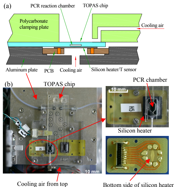
Figure 1: An illustration (a) and a top view (b) of the thermal cycling platform.
